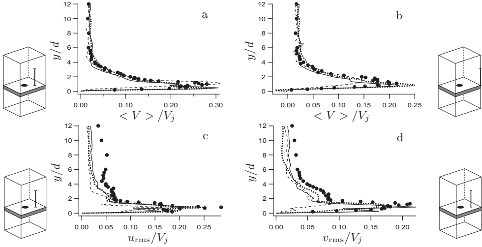
FIGURE 5. Velocity profiles: comparison between experimental results ( \bullet ), Run A ( --- ), Run B ( --- ) and Run C ( \cdots ). (a): time-averaged vertical velocity at station (c), x = 2.92 d , (b): time-averaged vertical velocity at station (d), x = 5.84 d , (c): streamwise RMS velocity at station (c), x = 2.92 d , (d): vertical RMS velocity at station (c), x = 2.92 d .
