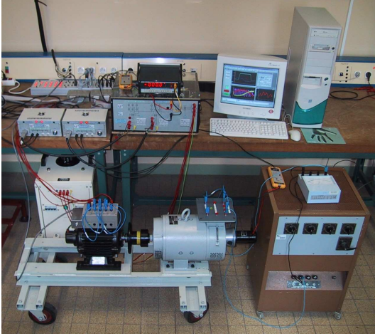
Fig. 9. Experimental bench
