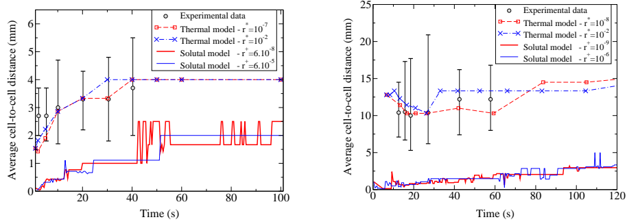
Figure C.9: Time evolution of the average cell-to-cell distance for thermal model, solutal model, and experiments. Left: Test case 1, Right: Test case 2. Error bars in experimental results reflect the size dispersion of the cells.
