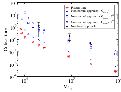
Figure C.6: Times t_{on}^* of convection onset obtained as a function of Marangoni numbers Ma_{th} using different approaches: t_{on}^{*(fr)} given by the frozen-time approach ; t_{on}^{*(nn)} given by the non-normal approach with E_T norm and different thresholds G_{thres} ; t_{on}^{*(nl)} given by the nonlinear approach for different perturbation amplitudes ( 10^{-7} \leq r^* \leq 10^{-2} for Ma_{th} = 2 \times 10^4 , 10^{-9} \leq r^* \leq 10^{-4} for Ma_{th} = 9 \times 10^4 and Ma_{th} = 2.5 \times 10^5 ). The other dimensionless parameters are such that Ra_{th} = 0 , Bi = 0.01 . For non-normal and frozen-time methods, Prandtl number is set to Pr = \infty , for the nonlinear approach, it is set to Pr = 100 .
