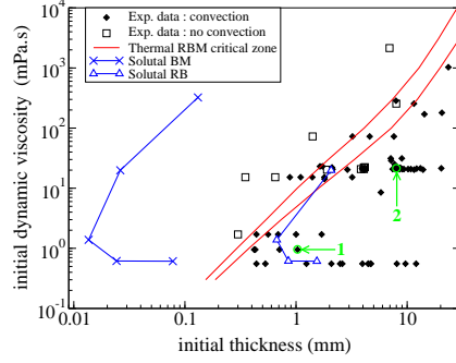
Figure C.8: Stability diagram for PIB/toluene solution (room temperature, v_{ev} \simeq 0.3 \mu\text{m.s}^{-1} , \Delta T_{st} \simeq 5 \text{ K} , H_{th} \simeq 28 \text{ W.m}^{-2}.\text{K}^{-1} ). The critical zone of the thermal Rayleigh-Bénard-Marangoni problem corresponds to the extreme boundaries obtained by the non-normal method formed by curves G_{thres} = 1 or G_{thres} = 100 using E_V or E_T norms (see Doumenc et al. [12]). The critical conditions of the solutal Bénard-Marangoni problem and the solutal Rayleigh-Bénard problem have been obtained by the nonlinear approach with r^+ = 10^{-6}/\Delta\varphi (see Trouette et al. [48]). Changing r^+ by \pm 2 decades results in a maximum variation of the critical thickness of the order of 30 % (not shown on the plot). Experimental test cases 1 and 2 are indicated by green circles and arrows.
