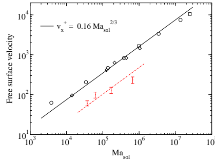
Figure C.12: Solutal Bénard-Marangoni problem: average dimensionless velocity at the free surface. Black open symbols: L2 norm from numerical simulations ( \circ : PIB/toluene, \varphi_{pi} = 0.047 , A = 5 , constant viscosity ; \square : PIB/toluene, A = 10 , variable viscosity ; \diamond : PS/toluene, A = 30 , variable viscosity ; Straight line: scaling law (B domain, prefactor fitted over numerical simulations) ; Error bars: experimental data from Bassou and Rharbi [2].
