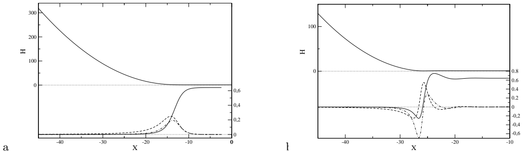
FIG. 7: Normal and tangential force distribution in the front and r^* meniscus, in dimensionless units. (a) Upper graph: Front meniscus profile. Lower graph: solid line: pressure P = 0.643 - H''(X) ; dashed line: meniscus contribution to the viscous stress (H - 1)/H^2 ; dot-dashed line: velocity divergence -H'/H^2 . (b) Same functions for the rear meniscus r^* . Full line: P = 0.643 - H''(X) ; dashed line: (1)
