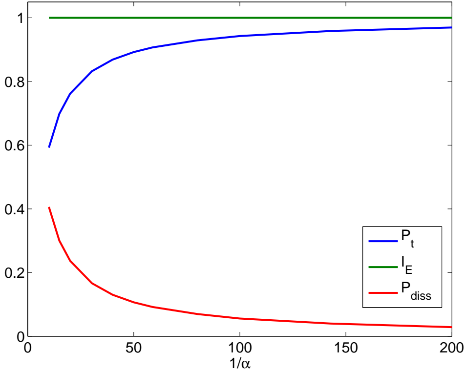
Fig. 5 Stationary energy balance for the fluctuations, in the case of a parabolic base profile in a channel geometry, with k = l = 1 and different values of the friction coefficient \alpha . We see that in the inertial limit \alpha \ll 1 , all the energy injected in the fluctuations is transferred to the zonal flow, while the energy dissipated in the fluctuations vanishes.
