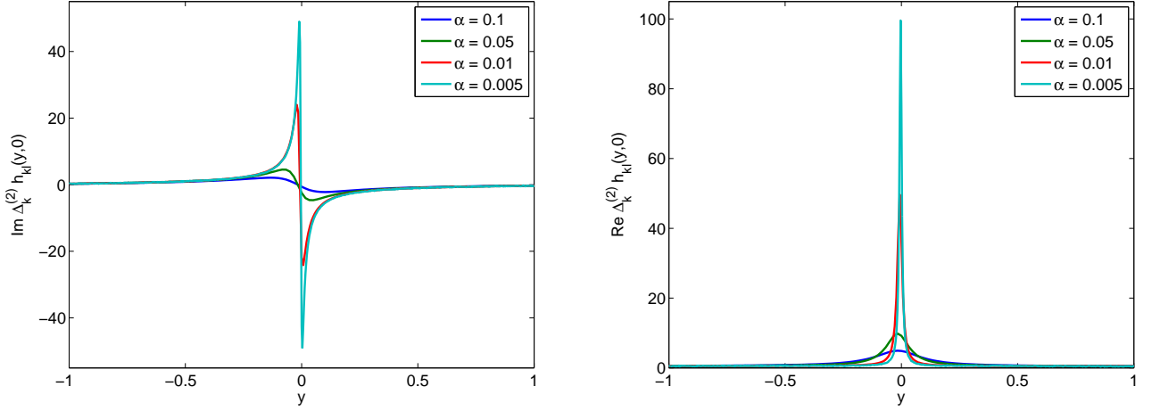
Fig. 2 Real and imaginary parts of the k -th Fourier component of the stationary vorticity auto-correlation function \Delta_k^{(2)} h_{kl}(y, y_2)|_{y_2=0} in the case of a parabolic base profile in a channel geometry, with k = l = 1 and different values of the friction coefficient \alpha . The plots clearly show the expected divergence at y = 0 .
