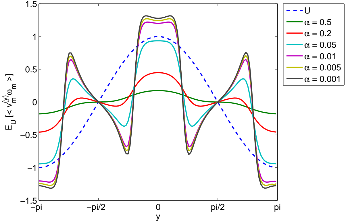
Fig. 4 The Reynolds stress divergence F(y) = \mathbb{E}_U \left[ \left\langle v_m^{(y)} \omega_m \right\rangle \right] = 2kc_{kl} \mathfrak{J}[h_{kl}(y,y)] in the case of a cosine base profile U(y) = \cos y in a periodic geometry, with k = 2, l = 0 and different values of the friction coefficient \alpha . Again, we observe the convergence of F towards a smooth function when \alpha \rightarrow 0 , even at the stationary points y = 0 and y = \pi where we do not have full theoretical predictions.
