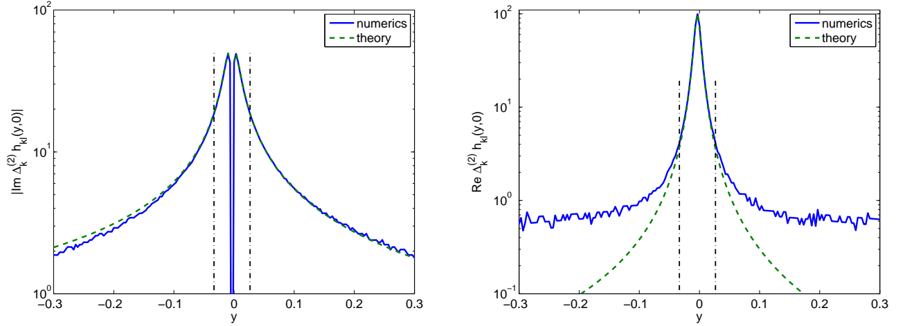
Fig. 3 Divergence of the stationary vorticity auto-correlation function \Delta_k^{(2)} h_{kl}(y, y_2)|_{y_2=0} near y = 0 , in the case of a parabolic base profile in a channel geometry, with k = l = 1 and \alpha = 0.005 . As expected, the comparison between the numerical result and the universal shape (87) is very good in the range 1 \gg y \gg \frac{2\alpha}{ks_0} \simeq 0.006 (the area between the vertical lines).
