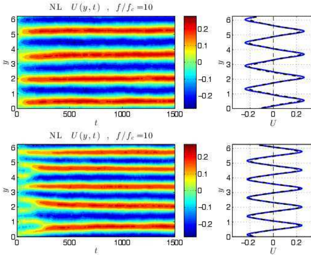
Fig. 7 Evolution of the zonally averaged velocity profile as obtained from non-linear simulations (left) and comparison of the stationary velocity profile obtained from non-linear simulations and from the deterministic part of the kinetic equation (88), or equivalently SSST [24, 18, 25]. The upper and lower pictures are obtained for the same values of the physical parameters but with different initial conditions. The figure shows that for a given set of parameters it can converge towards two attractors, U_0 and U_1 . Courtesy N. Constantinou.
