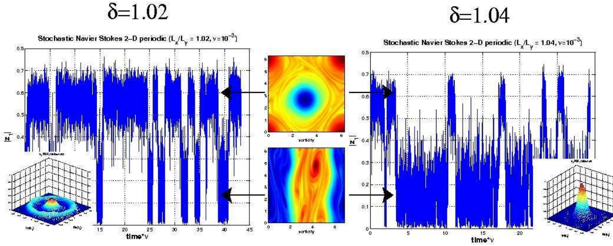
Fig. 6 Figure taken from [8] showing rare transitions (illustrated by the Fourier component of the largest y mode) between two large scale attractors of the periodic 2D Navier-Stokes equations. The system spends the majority of its time close to the vortex dipole and zonal flow configurations.
