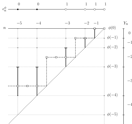
Figure 2: The next-jump time process (Y_n)_{n \leq 0} . The value of Y_n is shown by the bold interval.
