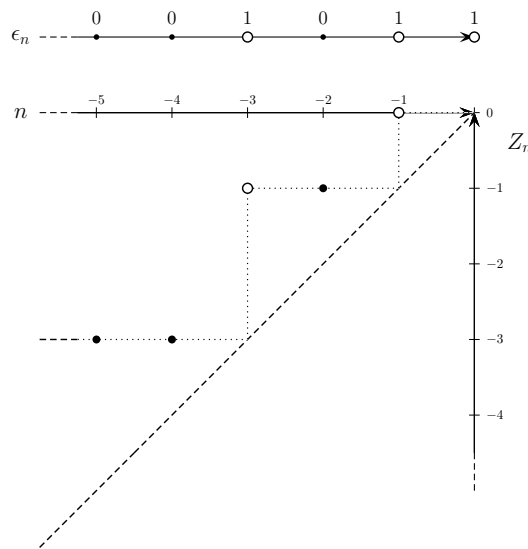
Figure 1: The next-jump time process
