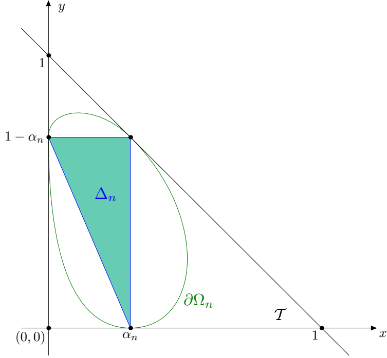
FIGURE 3. The \Omega_n are convex sets included in a fixed triangle
