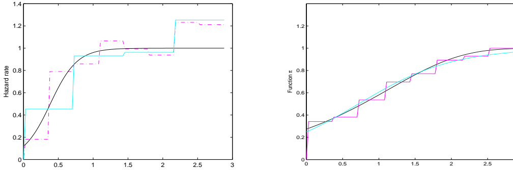
FIGURE 1. Strategy involving estimation of \pi : Left-side: True hazard rate (black line) for Model 2 and its estimators \hat{\lambda}_{\hat{m}(2)}^{(2)} with both nonparametric (magenta dotted line) and logit (cyan plain line) estimators of \pi . Right-Side: True auxiliary function \pi (black line) and its nonparametric (magenta) and logit (cyan) estimators. n = 1000 with \simeq 30\% censoring and 45% missing indicators.
