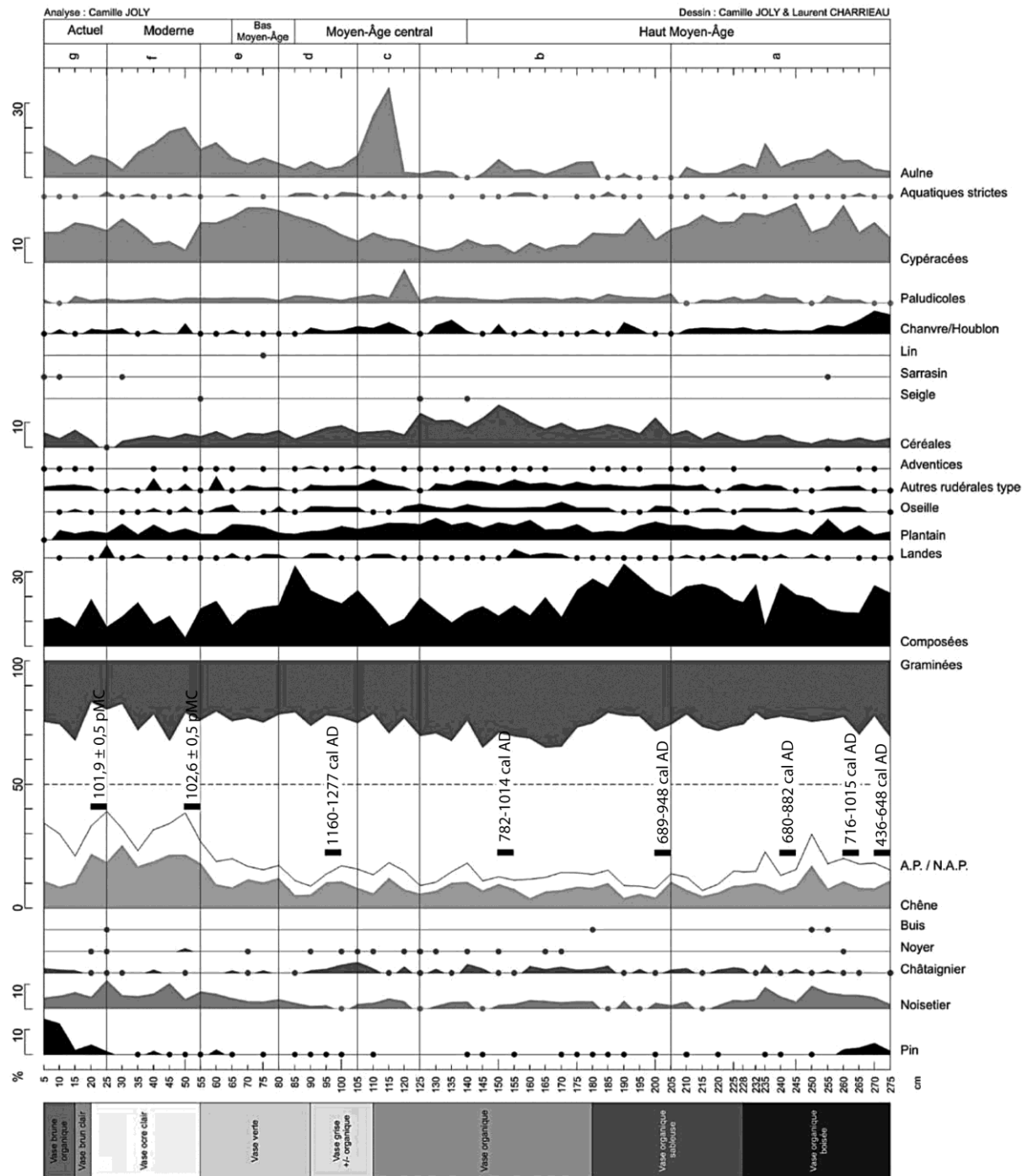
Figure 6 : Diagramme palynologique synthétique des Naudières – Synthetic palynological diagram from "Les Naudières" core.
