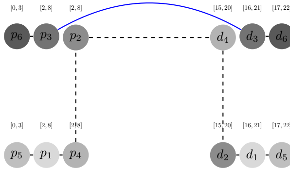
Figure 1: A solution without transfer (DARP)
