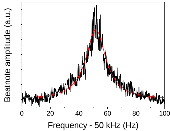
Figure 4. Down-converted beatnote of two independent \text{CO}_2 lasers, one stabilised on an \text{OsO}_4 resonance line, the other phase-locked to a comb repetition rate high-harmonic; red line is a Lorentzian fit of linewidth 17 Hz
