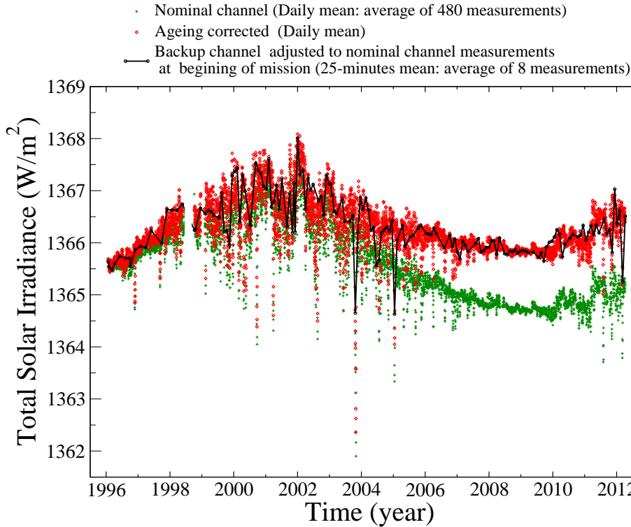
Figure 10. Temporal variation of TSI measurements from VIRGO/DIARAD. Green symbols: daily mean TSI measurements from the left channel; Black curve the 25-minutes average of the TSI measurements made each month with the right channel; Red symbols the daily mean aging-corrected TSI measurements.
