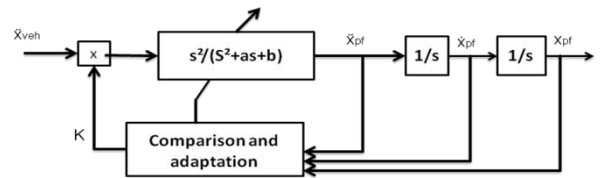
Figure 4. Schematic of the adaptive washout algorithm
