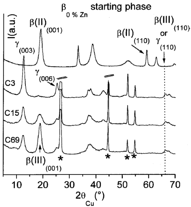
Figure 4. XRD patterns of the electrodes, after the n th charges ( C_n ), in comparison with that of the starting \beta_{0\%Zn} phase. Stars show the diffraction lines of Ni and C added to the electroactive material.
