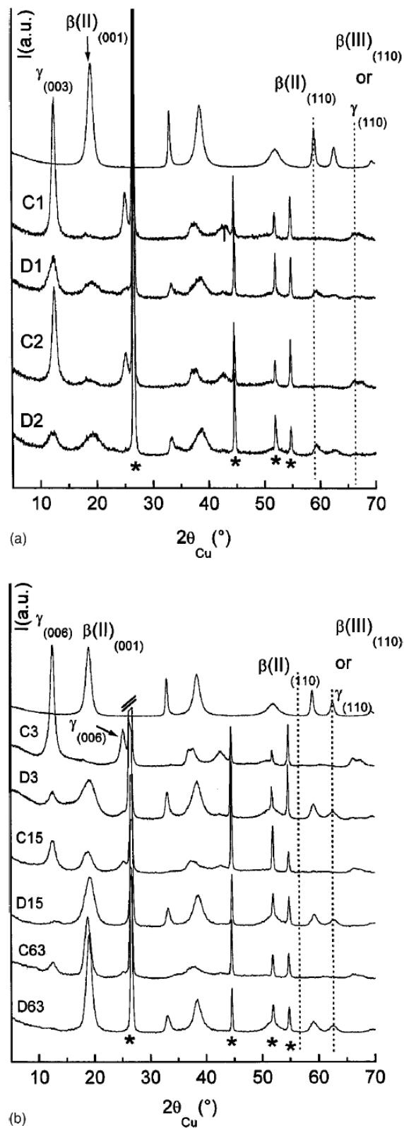
Figure 3. XRD patterns of the electrodes: (a) after the first and second charges (C1 and C2) and discharges (D1 and D2); (b) after the n th charges ( C_n ) and the n th discharges ( D_n ), in comparison with that of the starting \beta_{6\%Zn} phase. Stars show the diffraction lines of Ni and C, added to the electroactive material.
