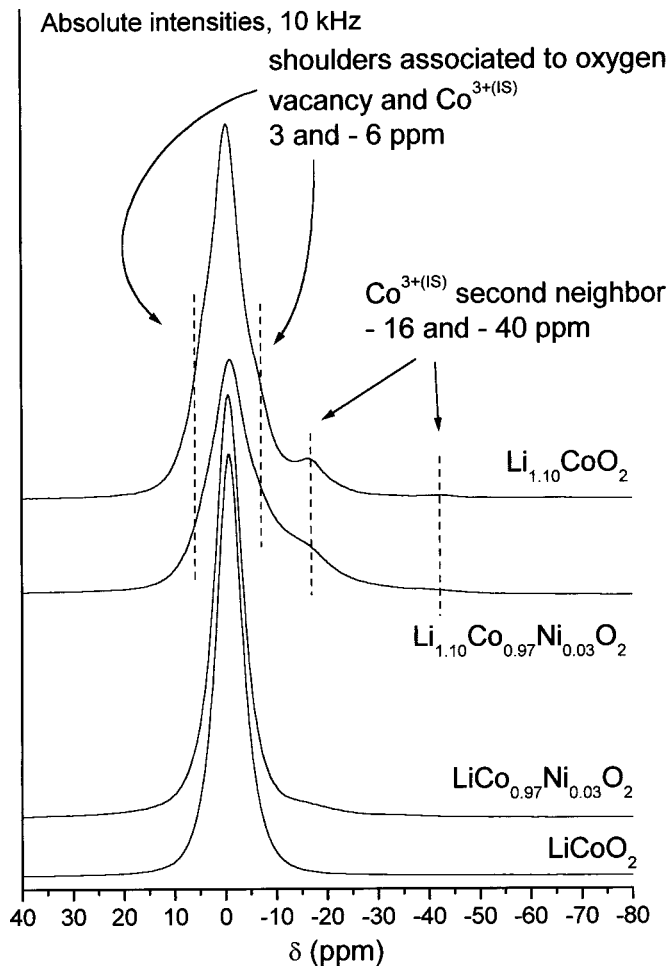
Figure 11. Expansion of the central signal of 10 kHz {}^7\text{Li} MAS NMR spectra for the various \text{Li}_{x_0}\text{Co}_{1-y}\text{Ni}_y\text{O}_2 phases ( x_0 = 1.0, 1.10 ; y = 0.0, 0.03 ).
