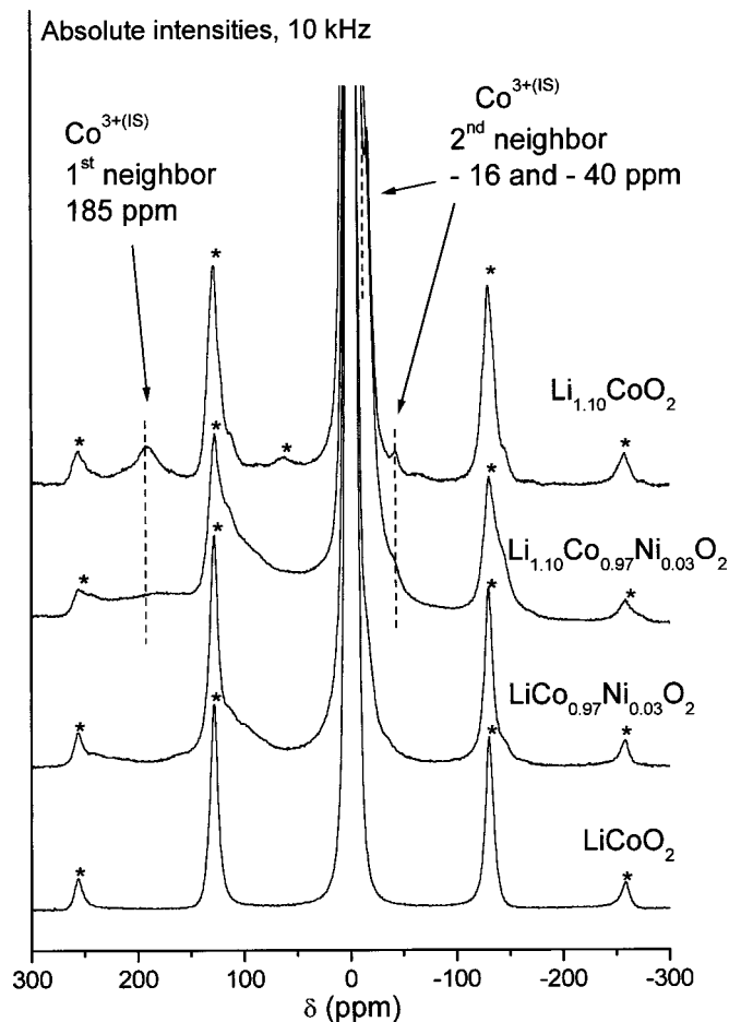
Figure 10. 10 kHz {}^7\text{Li} MAS NMR spectra for the various \text{Li}_{x_0}\text{Co}_{1-y}\text{Ni}_y\text{O}_2 phases ( x_0 = 1.0, 1.10 ; y = 0.0, 0.03 ), (* = spinning side bands).
