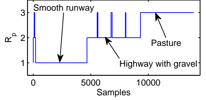
Fig. 6. Validation of the road detection mechanism when the suspension is submitted to the three roads.
