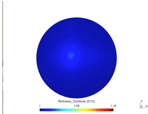
Figure 7: Evolution of Wealth Density \mathcal{W} . (Animation available on YouTube: http://youtu.be/05JNyznPxxvw .)
