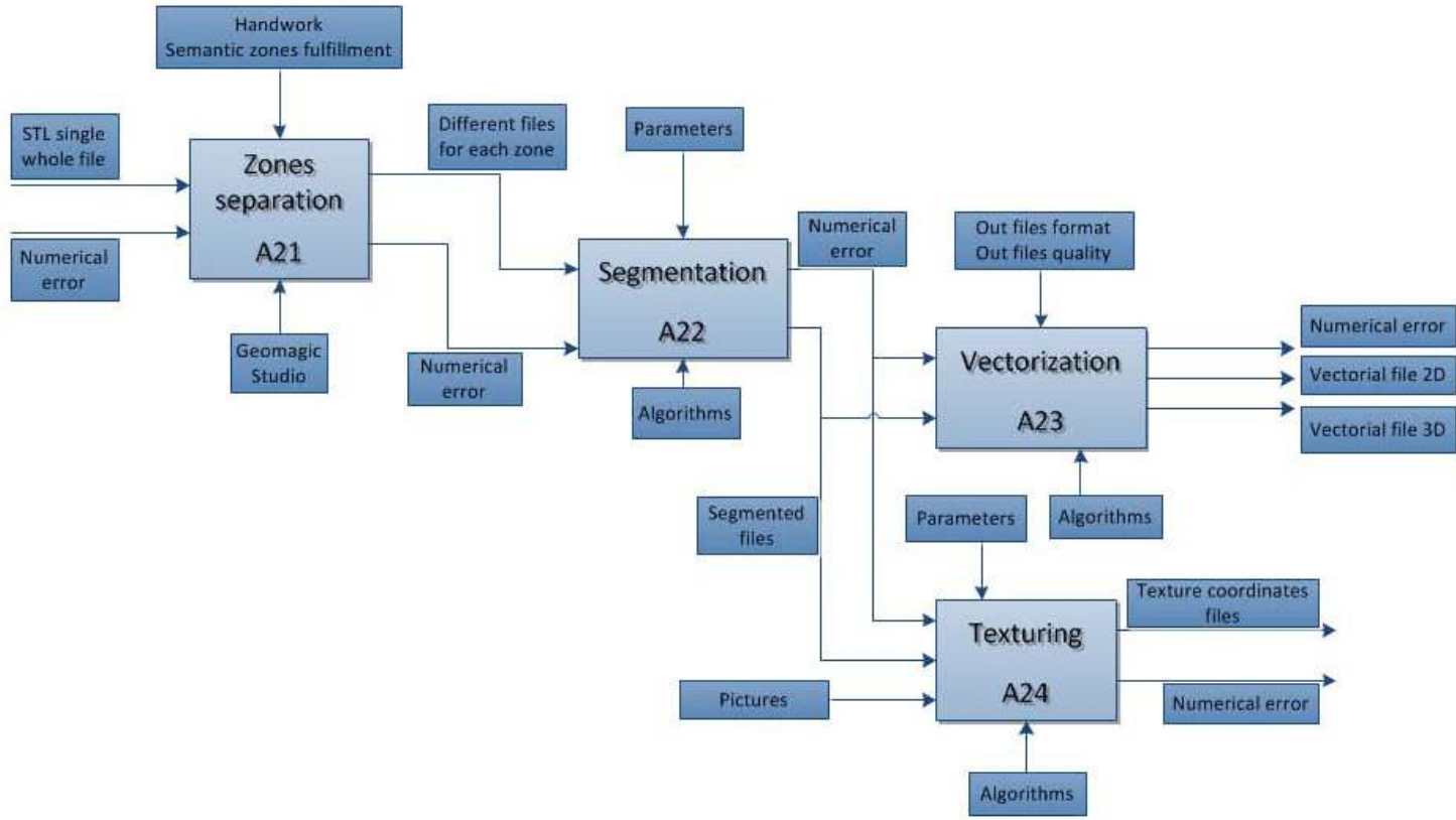
fig 5: SADT A2 diagram: zoning (A21), segmentation (A22) and vectorization (A23)
