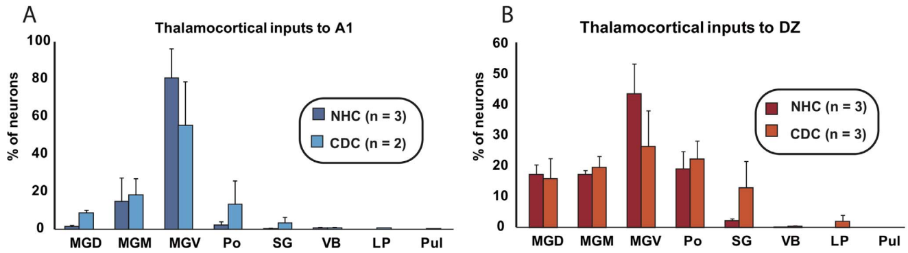
Figure 4. Histograms of the means of the distribution (in % of total, \pm se) of projecting cells in the thalamic nuclei following an injection in A1 (A) or DZ (B). Values for normal (NHC) and deaf (CDC) cats are presented separately. No striking differences are observed in the proportions beside an abnormal projection in the deaf cats from the Lateral Posterior nucleus (LP) to A1. The number of injections sites in each group is indicated (n).
