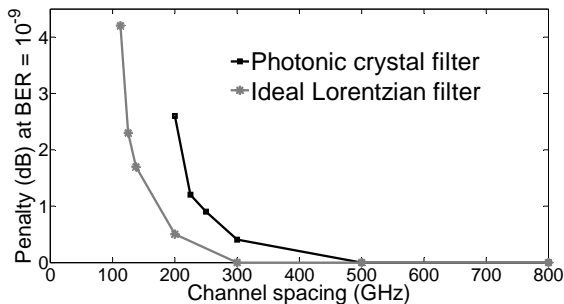
Fig. 5. Power penalty as a function of channel spacing.
