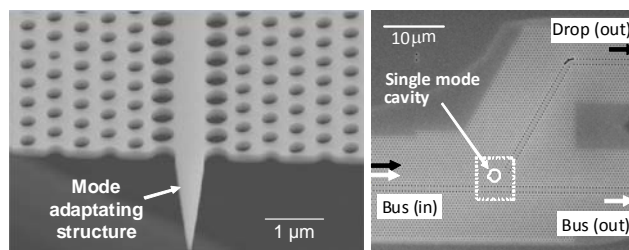
Fig. 1. SEM picture of the WDM filter: detail of the membrane with mode adapter structure (left), filter with the drop channel (right).
