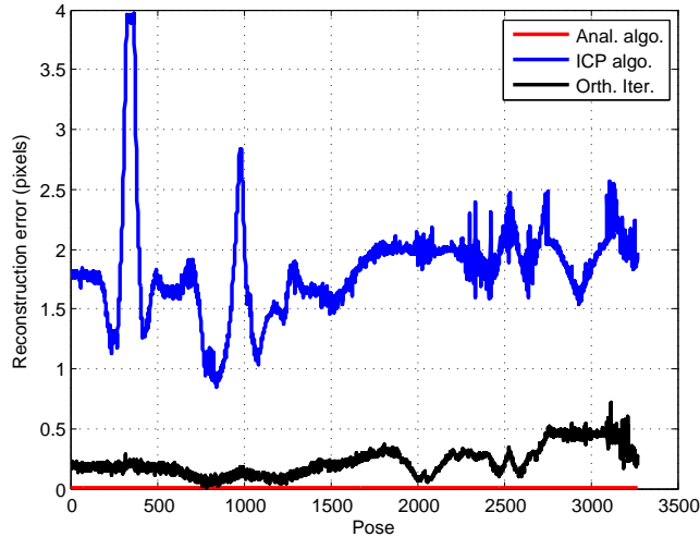
Figure 10 Reconstruction error.
