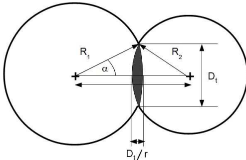
FIG. 4. Scheme of interconnection.
