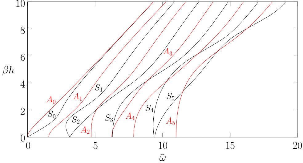
Figure 2: Dispersion curves, derived from the dispersion relation \frac{\omega^4}{c_s^4} = 4\beta^2\alpha_s^2 \left(1 - \frac{\alpha_p \tan(\alpha_p h + \kappa)}{\alpha_s \tan(\alpha_s h + \kappa)}\right) , with \alpha_p = \sqrt{\beta^2 - \frac{\omega^2}{c_p^2}} and \alpha_s = \sqrt{\beta^2 - \frac{\omega^2}{c_s^2}} and where c_p = \sqrt{\frac{\lambda+2\mu}{\rho}} is the longitudinal (pressure) wave velocity and c_s = \sqrt{\frac{\mu}{\rho}} is the shear wave velocity, for symmetric ( \kappa = 0 , in black) and antisymmetric ( \kappa = \frac{\pi}{2} , in red) propagative Rayleigh–Lamb modes in a plate of thickness 2h made of a material with Poisson’s ratio \nu equal to 0.33 (aluminium for instance), the dimensionless variable \tilde{\omega} being equal to \frac{\omega h}{c_s} . Inspection of the second and fifth curves associated with the symmetric modes reveals that backward propagating modes exist at low frequencies.
