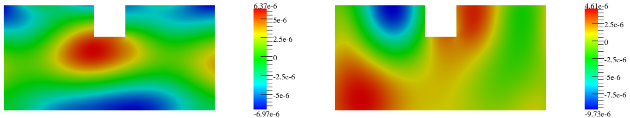
Figure 8: Real parts of the horizontal (on the left) and vertical (on the right) components of the reference solution computed using transparent boundary conditions (see [14]).
