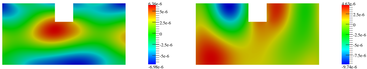
Figure 10: Real parts of the horizontal (on the left) and vertical (on the right) components of the reference solution computed using perfectly matched layers and the novel approach with \mathcal{N}_\epsilon = 5 .
