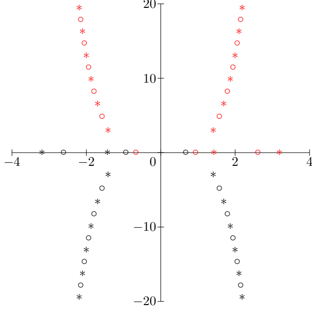
Figure 3: Positions in the complex plane of the first wavenumbers \pm\beta_n respectively associated with rightgoing (in red) and leftgoing (in black) Rayleigh–Lamb modes (the symbols \circ (resp. * ) refer to symmetric (resp. antisymmetric) modes) in an aluminium ( \rho = 2700 \text{ kg m}^{-3} , E = 69 \text{ GPa} , and \nu = 0.33 ) plate of thickness 2 m at low frequency ( \omega = 8833.7825 \text{ rad s}^{-1} ). Two wavenumbers are associated to backward propagating symmetric modes.
