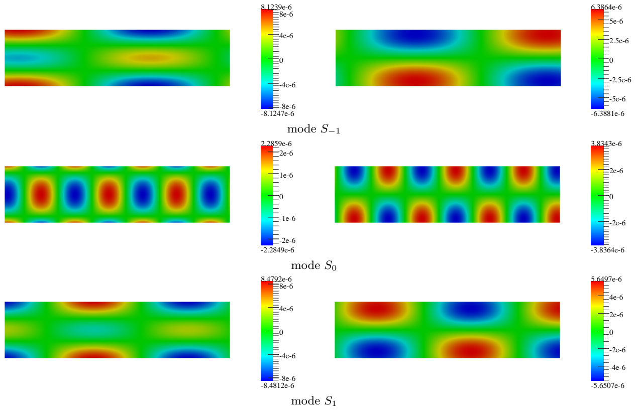
Figure 4: Real parts of the horizontal (on the left) and vertical (on the right) components of the symmetric propagative Rayleigh–Lamb modes for \omega = 8833.7825 \text{ rad s}^{-1} in a plate of thickness 2 m made of aluminium.
