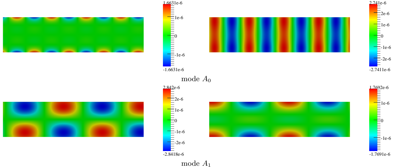
Figure 5: Real parts of the horizontal (on the left) and vertical (on the right) components of the antisymmetric propagative Rayleigh–Lamb modes for \omega = 8833.7825 \text{ rad s}^{-1} in a plate of thickness 2 m made of aluminium.
