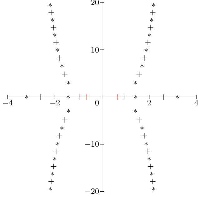
Figure 3: Positions in the complex plane of the first wavenumbers \pm\beta_n respectively associated with rightgoing and leftgoing Rayleigh–Lamb modes (the symbols + (resp. *) refer to symmetric (resp. antisymmetric) modes) in an aluminium plate of thickness 2 m at low frequency ( \tilde{\omega} = 2.85 ). The wavenumbers of the backward propagative modes are drawn in red.
