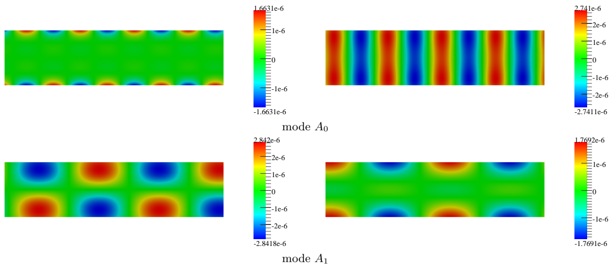
Figure 5: Real parts of the two components of the antisymmetric propagative Rayleigh-Lamb modes for \omega = 8833.7825 \text{ rad s}^{-1} in a plate of thickness 2 m made of aluminium.
