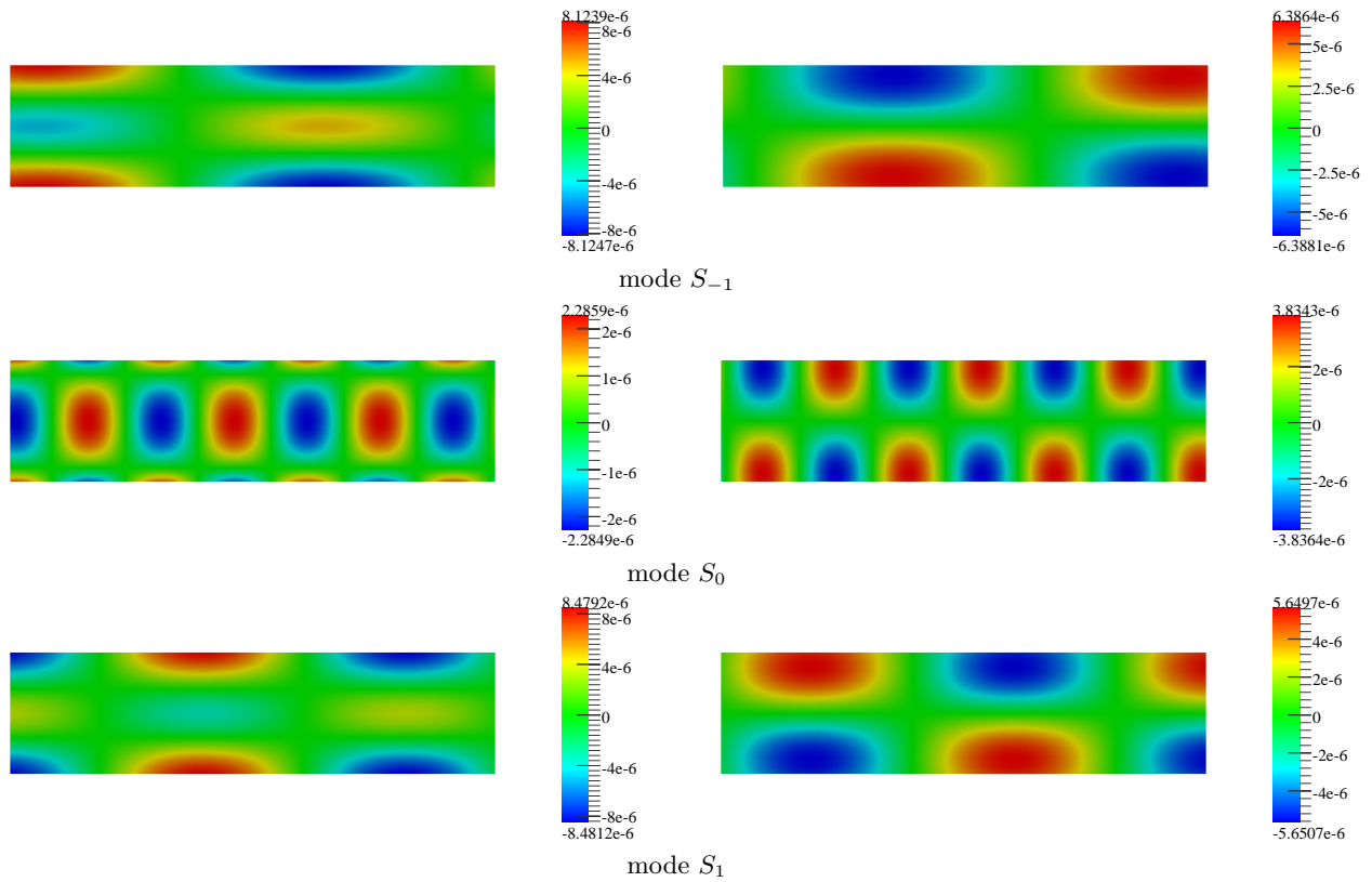
Figure 4: Real parts of the two components of the symmetric propagative Rayleigh-Lamb modes for \omega = 8833.7825 \text{ rad s}^{-1} in a plate of thickness 2 m made of aluminium.
