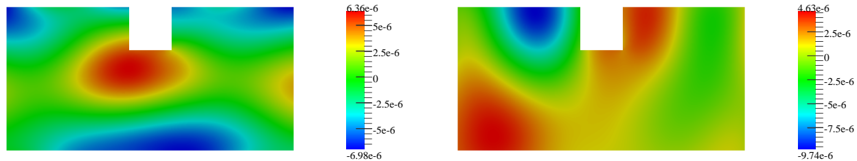
Figure 10: Real parts of the two components of the reference solution computed using perfectly matched layers and the novel approach with \mathcal{N}_\epsilon = 5 .
