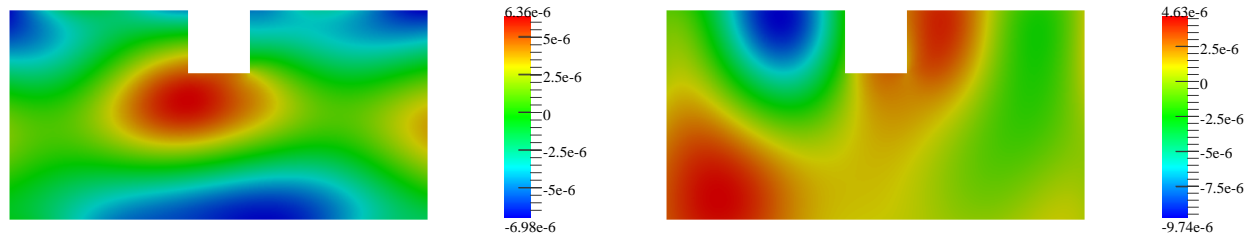
Figure 10: Real parts of the two components of the reference solution computed using perfectly matched layers and the novel approach with \mathcal{N}_\epsilon = 5 .
