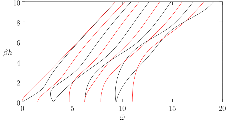
Figure 2: Dispersion curves for symmetric (black lines) and antisymmetric (red lines) propagative Rayleigh–Lamb modes in a plate of thickness 2h made of a material with Poisson’s ratio \nu equal to 0.33 (aluminium for instance), the dimensionless variable \tilde{\omega} being equal to \frac{\omega h}{c_s} , where c_s = \sqrt{\frac{\mu}{\rho}} is the shear wave velocity. One observes that the second and fourth symmetric modes are backward at low frequencies.
