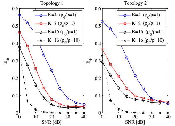
Fig. 3. E_\Phi vs. SNR performance.
