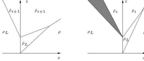
FIGURE 5. With reference to Example 2, the solutions \rho_{\bar{t},1} and \rho_{\bar{t},3} . Above \check{\rho}_L = \check{\rho}(f(\rho_L)) .
