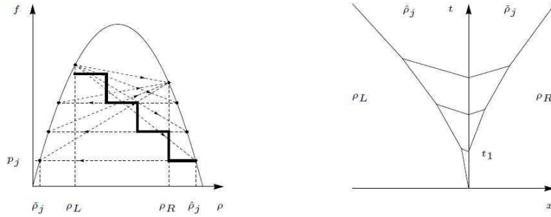
FIGURE 3. Construction of a non self-similar entropy weak solution as in Example 1. On the left, the thick line corresponds to the efficiency of the exit p|_{\rho_L, \hat{\rho}_j} \cdot .
