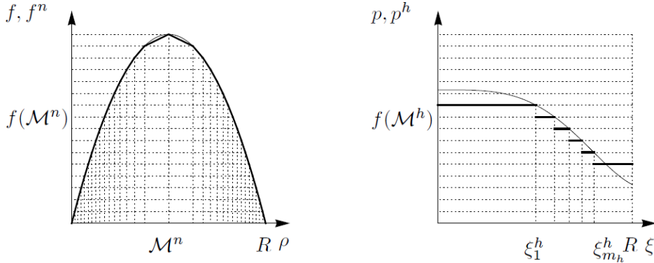
FIGURE 2. Left: : In thin line f and in thick line the approximation f^n . Right: In thin line p and in thick line the approximation p^h .
