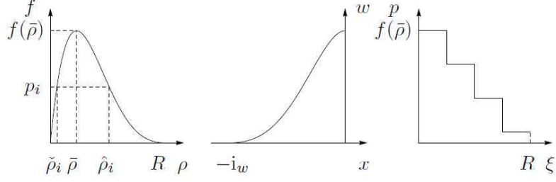
FIGURE 1. Examples of functions satisfying conditions (F) , (W) , (P0) and (P2) .
