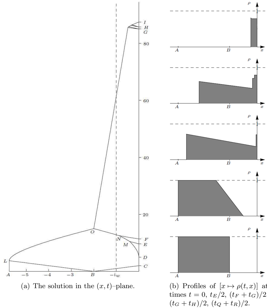
FIGURE 7. The solution described in Sec. 5 and corresponding to the choice (32)
