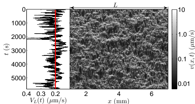
FIG. 1. Right: The spatio-temporal velocity field v(x,t) during a fracture experiment. Left: The corresponding spatially averaged signal V_L(t) = \langle v(x,t) \rangle_L , over the full system size L . The solid red line indicates the full space-time average velocity \langle V_L \rangle_T = \bar{v} .
