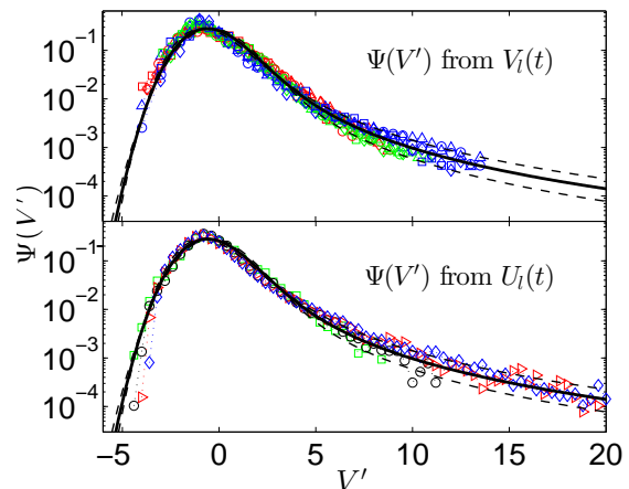
FIG. 3. (Color online) PDF \Psi(V') of the global velocity V_i(t) (upper panel) for three different experiments (red, green, and blue), at four different averaging scales l/x^* \in \{40, 20, 13, 10\} , in semi-log representation. For one of these experiments (blue), we obtain \Psi(V') from U_i(t) , smoothed over 15 time steps, at the same averaging scales (lower panel). The solid lines show the PDF \Psi(V'; 1.7, 1) , obtained from Eq. (5), whereas the dashed lines correspond to \Psi(V'; 1.7 \pm 0.1, 1) , displaying the effect of the variations in \alpha .
