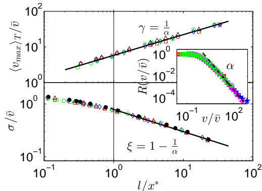
FIG. 2. Average maximum velocity (upper panel) \langle v_{max}^l \rangle_T / \bar{v} and standard deviation (lower panel) \sigma / \bar{v} of V_i(t) , as function of the measuring window rescaled by the correlation length, l/x^* . The upper solid line corresponds to the slope \gamma = 1/1.7 \approx 0.58 . The lower solid line is a fit of Eq. (4) for l/x^* > 3 , giving \xi = 0.42 \pm 0.03 and thus \alpha = 1.7 \pm 0.1 . Circular black markers show, for one experiment, \sigma(l) , obtained from U_i(t) (smoothed over 15 time steps) as defined in the text. The inset shows the cumulative PDF of the local velocity R(v/\bar{v}) . The dashed line is a fit to the asymptotic tail, using \alpha = 1.7 , to obtain \lambda^+ as defined in the text.
