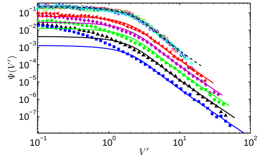
FIG. 4. (Color online) PDFs \Psi(V') for one experiment in log-log representation, at the scales l/x^* \approx \{40, 20, 13, 10\} (upper collapsed curves, empty markers), and in filled markers from top to bottom, at l/x^* \approx \{3, 1, 0.5, 0.2, 0.05\} respectively. The latter distributions with the theoretical curves, \Psi(V'; 1.7, 1) shown as solid lines, have been shifted for visual clarity.
