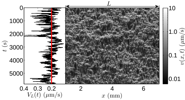
FIG. 1. Right: The spatio-temporal velocity field v(x, t) during a fracture experiment. Left: The corresponding spatially averaged signal V_L(t) = \langle v(x, t) \rangle_L , over the full system size L . The solid red line indicates the full space-time average velocity \langle V_L \rangle_T = \bar{v} .
