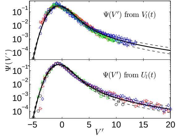
FIG. 3. (Color online) PDF \Psi(V') of the global velocity V_l(t) (upper panel) for three different experiments (red, green, and blue), at four different averaging scales l/x^* \in \{40, 20, 13, 10\} , in semi-log representation. For one of these experiments (blue), we obtain \Psi(V') from U_l(t) , smoothed over 15 time steps, at the same averaging scales (lower panel). The solid lines show the PDF \Psi(V'; 1.7, 1) , obtained from Eq. (5), whereas the dashed lines correspond to \Psi(V'; 1.7 \pm 0.1, 1) , displaying the effect of the variations in \alpha .
