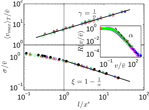
FIG. 2. Average maximum velocity (upper panel) \langle v_{max}^l \rangle_T / \bar{v} and standard deviation (lower panel) \sigma / \bar{v} of V_l(t) , as function of the measuring window rescaled by the correlation length, l/x^* . The upper solid line corresponds to the slope \gamma = 1/1.7 \approx 0.58 . The lower solid line is a fit of Eq. (4) for l/x^* > 3 , giving \xi = 0.42 \pm 0.03 and thus \alpha = 1.7 \pm 0.1 . Circular black markers show, for one experiment, \sigma(l) , obtained from U_l(t) (smoothed over 15 time steps) as defined in the text. The inset shows the cumulative PDF of the local velocity R(v/\bar{v}) . The dashed line is a fit to the asymptotic tail, using \alpha = 1.7 , to obtain \lambda^+ as defined in the text.
