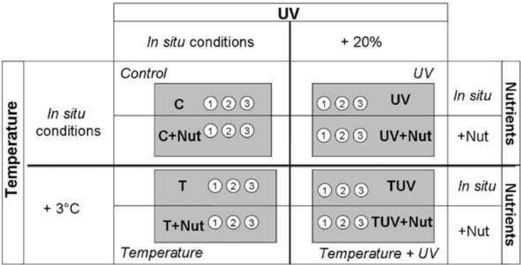
Figure 1 Crossed factorial experimental design conducted to assess the effects of the three regulatory factors: (Temperature, UVB radiation and nutrient increases).
