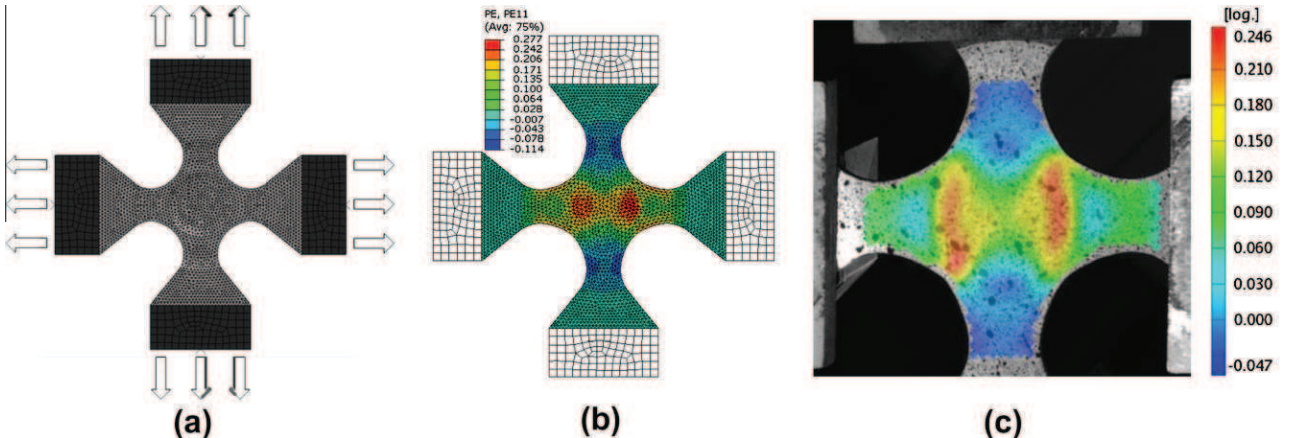
Fig. 10. (a) Numerical model of biaxial test, (b) numerical results of strain distribution in cruciform specimen and (c) experimental strain map obtained by SIC method.
