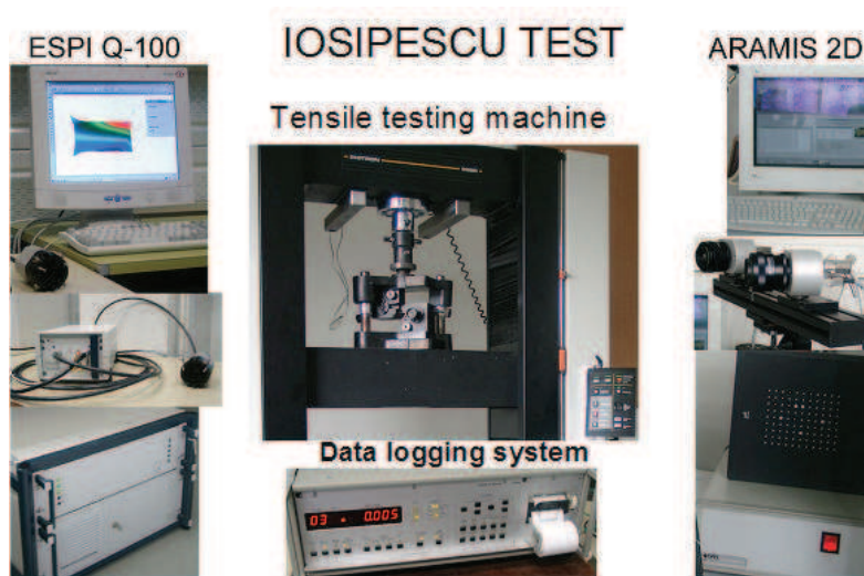
Fig. 15. Testing device
