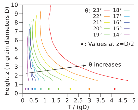
FIG. 15. (Color online) Vertical profile of the velocity fluctuations, averaged over y .
