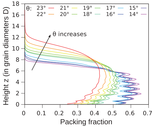
FIG. 6. (Color online) Height-averaged packing fraction (smoothed over \pm 0.5D in z ) for each angle of inclination. The layering is clearly apparent at low angles and disappears in the presence of the secondary flows.
