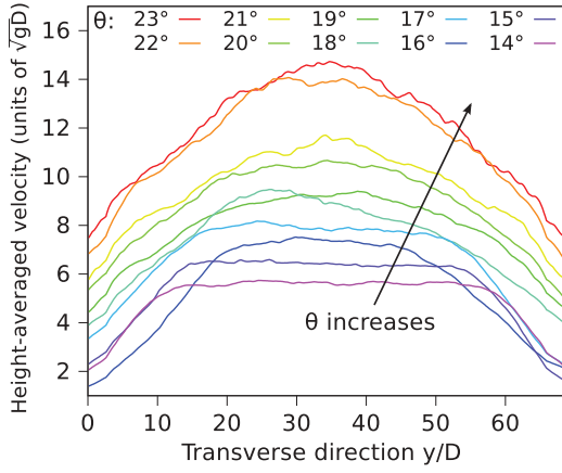
FIG. 12. (Color online) Transverse velocity profile, smoothed over \pm 2.5D in y , averaged over z .
