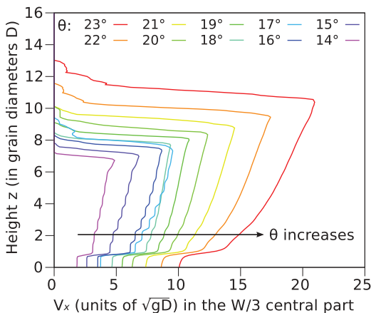
FIG. 13. (Color online) Height profile of the velocity along x averaged over the central part of the flow.
