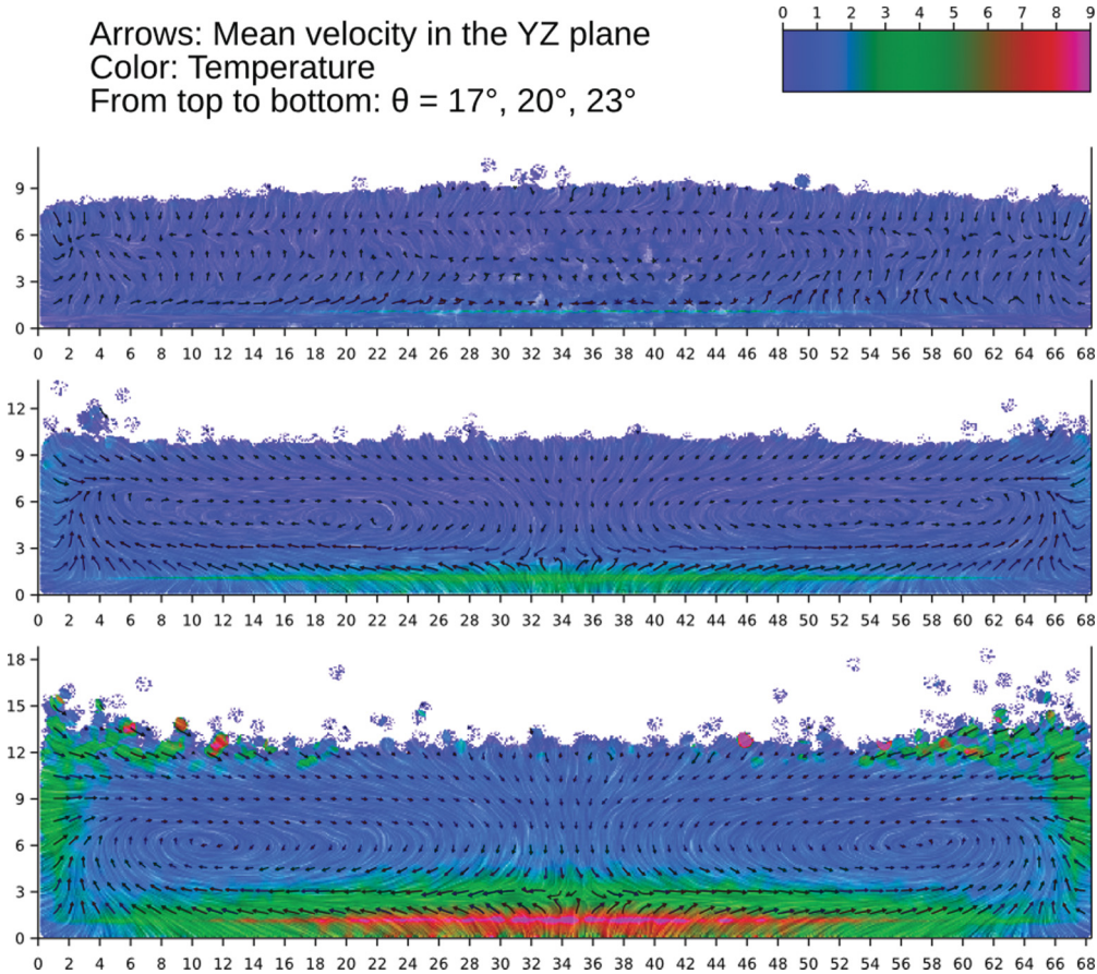
FIG. 17. (Color online) Vector field of the velocities in the transverse yz plane on top of the color (gray) -coded “granular temperature” T . The data, obtained in the steady and fully developed regime, have been averaged over time and over the periodic cell in the direction of the flow.
