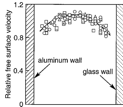
FIG. 1. Top view of free surface velocity profiles for granular flows down flat and frictional base (reprinted from Ref. [2]). The influence of the side walls is apparent over 2/3 of the flow width.
