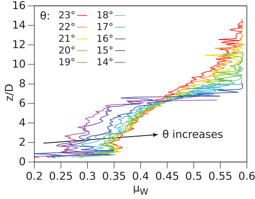
FIG. 9. (Color online) Friction coefficient profile on the lateral walls for several value of the inclination angle \theta .
