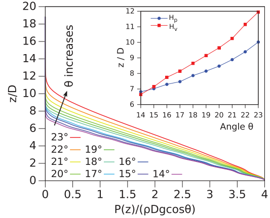
FIG. 10. (Color online) Main diagram: Vertical profiles of the averaged pressure for the hydrostatic approximation in the center part of the curves. Inset: The effective heights of the flows, with respect to the hydrostatic approximation H_p and maximal flow velocity H_v . See the main text.
