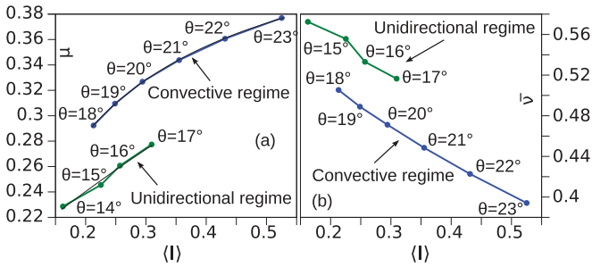
FIG. 20. (Color online) (a) Effective friction \mu and (b) average packing fraction \bar{v} vs average inertial number \langle I \rangle in the bulk of the flow. Overlaid thin black lines in (a) are the empirical fits mentioned in the main text.
