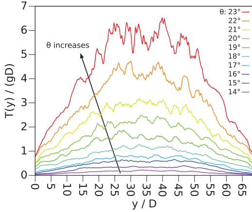
FIG. 16. (Color online) Transverse profile of the velocity fluctuations at the flat base, smoothed over \pm 2.5D in y .
