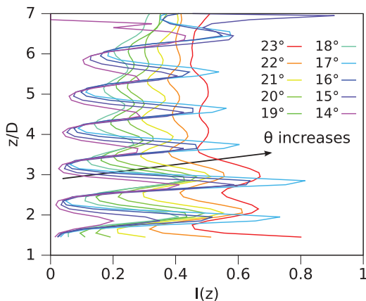
FIG. 18. (Color online) Vertical profile of the inertial number I .
