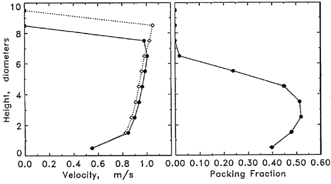
FIG. 2. Velocity (left) and packing fraction (right) profiles obtained by Walton [31] for moderate flow heights. Solid lines are instantaneous profiles, dotted line is time average profiles. Reprinted from Ref. [31].
