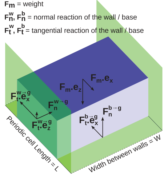
FIG. 8. (Color online) External forces balance on the grain flow.
