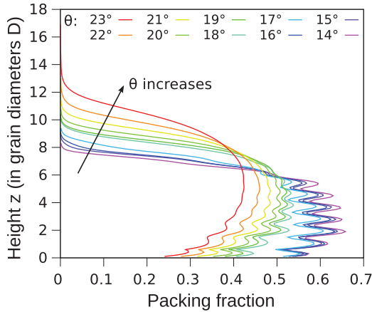
FIG. 6. (Color online) Height-averaged packing fraction (smoothed over \pm 0.5D in z ) for each angle of inclination. The layering is clearly apparent at low angles and disappears in the presence of the secondary flows.
