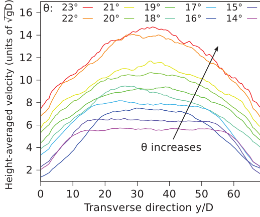
FIG. 12. (Color online) Transverse velocity profile, smoothed over \pm 2.5D in y , averaged over z .
