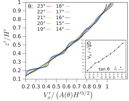
FIG. 14. (Color online) Main plot: Bagnold velocity profile collapse. Inset: effective “sliding” velocities of the main bulk of the flow with respect to the basal layer of rolling grains.
