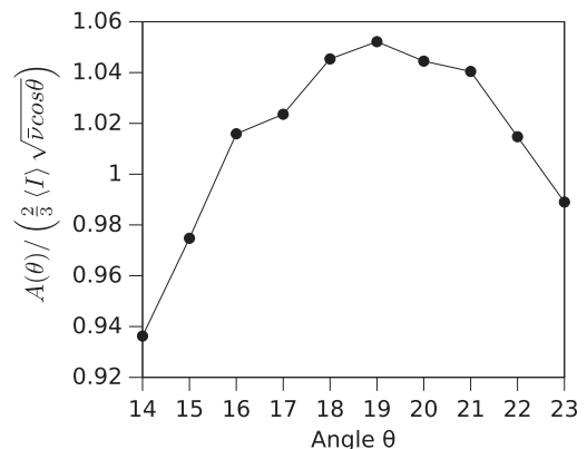
FIG. 19. Fit quality of the theoretical Bagnold profile for each angle.
