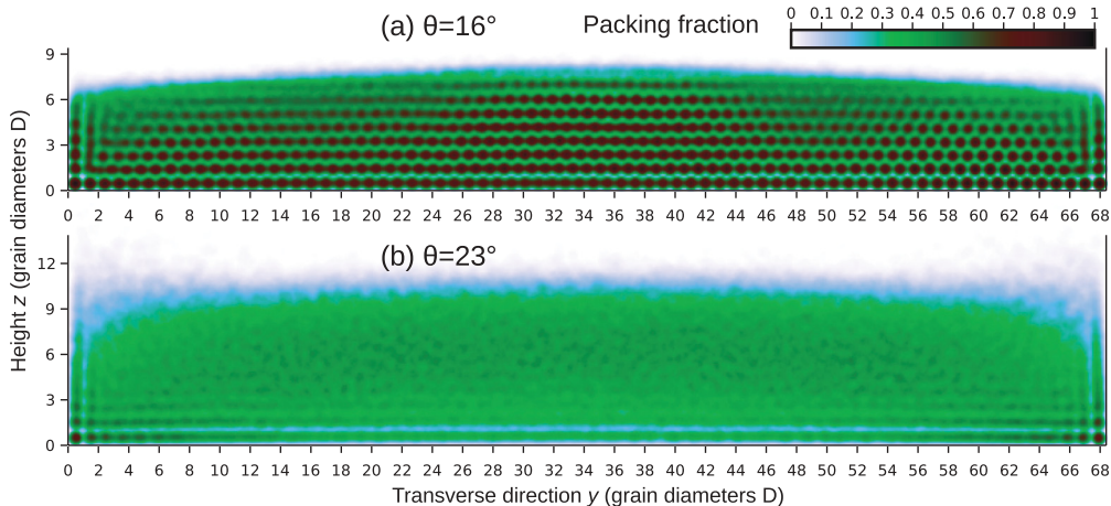
FIG. 7. (Color online) Packing fraction map, averaged over x . The layered structure at low angles disappears when granular convection takes place.
