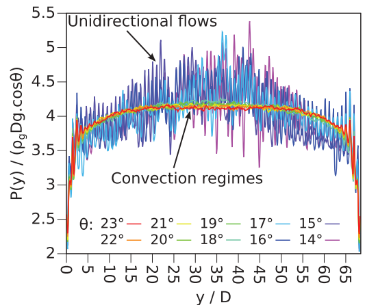
FIG. 11. (Color online) Normalized pressure computed from each contact with the base, smoothed over \pm 1D in y
