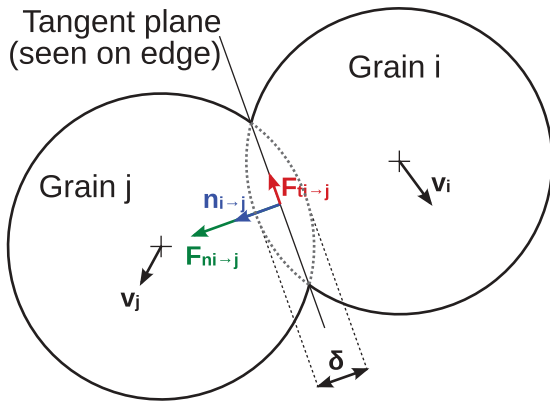
FIG. 3. (Color online) Overlapping spheres contact model. Grain i moves with a translation velocity v_i , and similarly for j . The force exerted by grain i on grain j during contact (characterized by the normal vector \mathbf{n}^{i \rightarrow j} ) is decomposed into a tangential component F_t^{i \rightarrow j} and a normal component F_n^{i \rightarrow j} . Both depend on the overlap \delta according to a contact model detailed in the main text.
