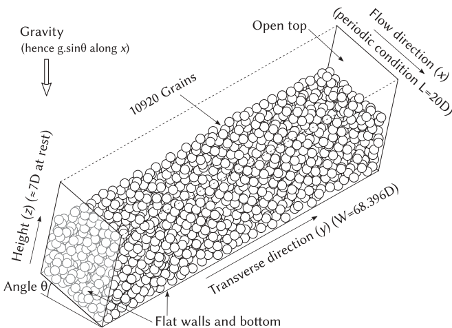
FIG. 4. Sketch of the MD simulation in a configuration corresponding to experiments [2] where an inclined plane is bounded by flat side walls and base.
