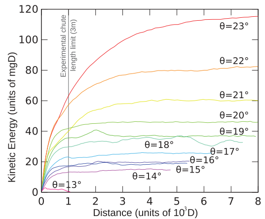
FIG. 5. (Color online) Translation kinetic energy vs distance traveled by the grains, showing regimes that appear accelerated within the chute length experimental limit, but reaching steady states at larger distances.
