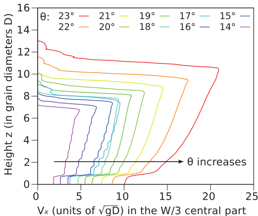
FIG. 13. (Color online) Height profile of the velocity along x averaged over the central part of the flow.
