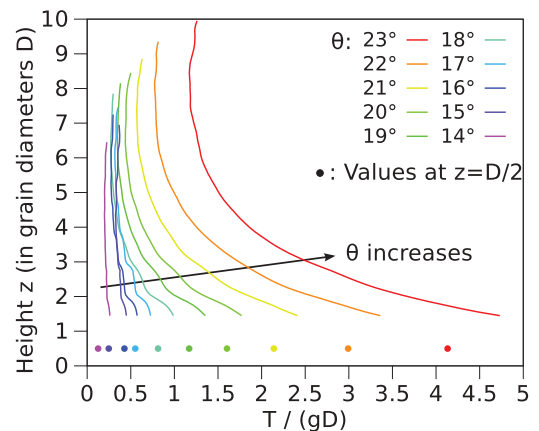
FIG. 15. (Color online) Vertical profile of the velocity fluctuations, averaged over y .
