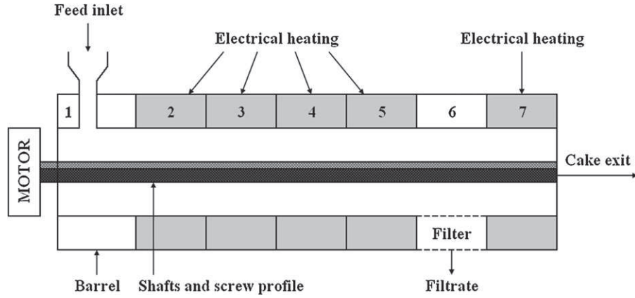
Fig. 1. Schematic modular barrel of the Cleextral BC 21 twin-screw extruder used for extraction of oil from jatropha seeds.
