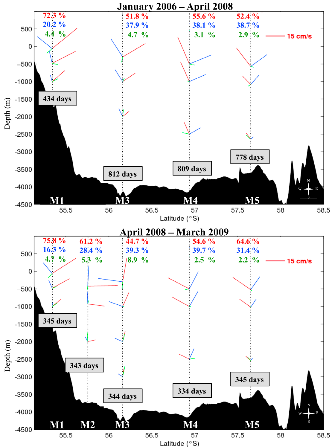
Figure 5. Empirical orthogonal functions (EOF) analysis of (top) the first period, 2006–2008, and of (bottom) the second period, 2008–2009. The first three EOFs for each mooring are plotted at the corresponding depths and latitude. The first EOF is plotted in red, the second in blue, and the third in green. The explained variance of each EOF is indicated by the corresponding color at the mooring position and the number of days of measurement in black. The bottom topography is indicated in solid black. Velocity scale is indicated in the upper right corner and compass directions in the lower right corner. The EOF analysis shown for M3 in the second period was performed with four instruments instead of five (i.e., without M3-2 at 500 m depth) to ensure coherence with the first period.
