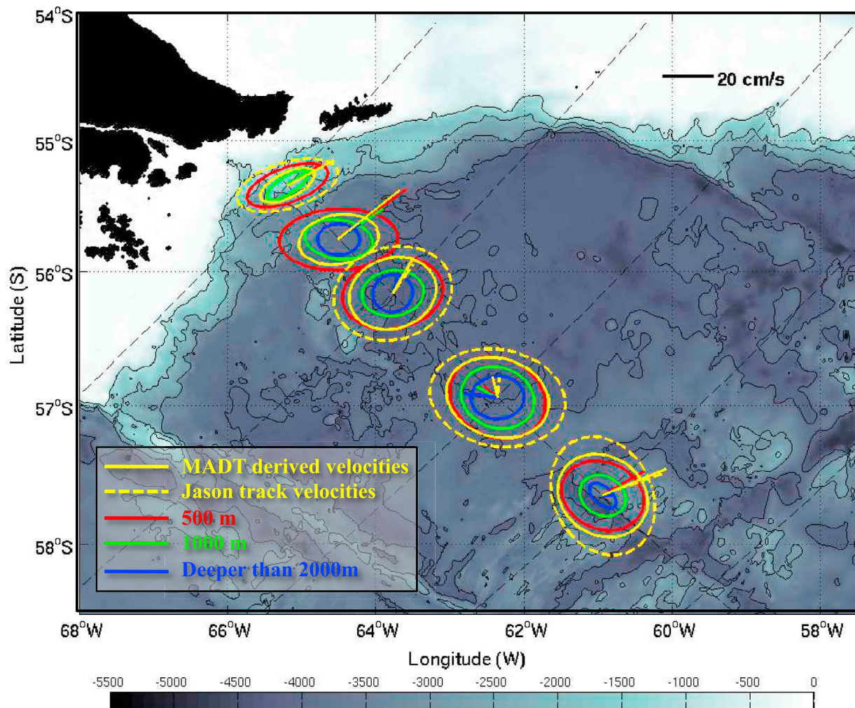
Figure 7. Mean and variance ellipses of the altimetrically derived surface velocities and the in situ velocities over the 3 year period: from 21 January 2006 to 1 April 2009. Surface velocities derived from maps of absolute dynamic topography (MADT) are shown by solid yellow lines and those derived from Jason 1 track data are shown by dashed yellow lines. M2 is not at an intersection of two Jason tracks and therefore no velocities have been computed from Jason 1 track data. Means and ellipses at different depths of the in situ velocities are plotted in red for 500 m depth, green for 1000 m depth, and blue for depths greater than 2000 m. Time resolution is 1 d for in situ velocities, 7 d for MADT-based velocities, and 10 d for Jason 1 track-based velocities. Bottom topography as in Figure 1.
