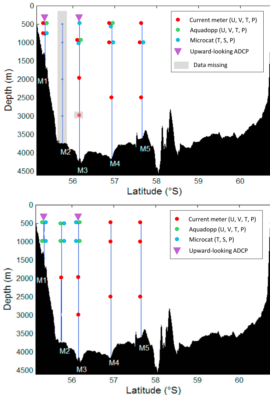
Figure 2. Vertical distribution of the instruments (top) in 2006–2008 and (bottom) in 2008–2009 along the mooring lines. Shaded instruments were lost or malfunctioning. Red dots indicate ANDERAA-type current meters, and green dots indicate Aquadopp-type acoustic current meters. Microcats are indicated by blue dots; the Microcats measure temperature, salinity, and pressure. Purple triangles indicate the position of the moored upward looking acoustic Doppler current profiler (ADCP).
