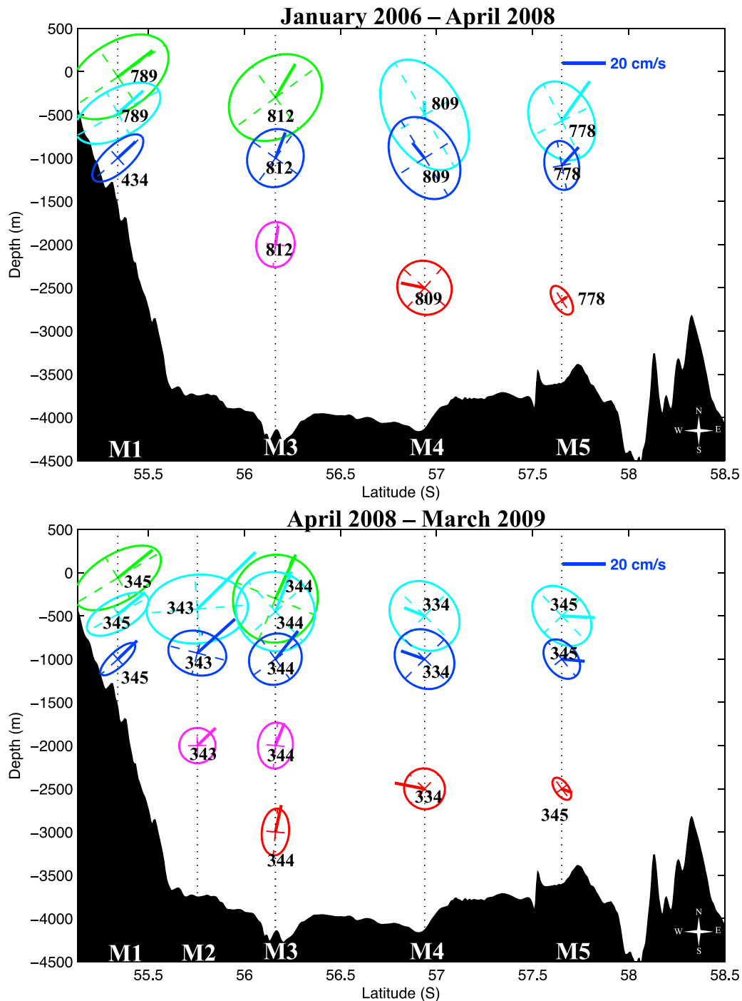
Figure 4. Mean velocities and variance ellipses for (top) the first period, 2006–2008, and for (bottom) the second period, 2008–2009. The number of days of measurement is indicated in black. The axes of the ellipses are plotted in a thin dotted colored line. Ellipses corresponding to the level of the upward looking ADCP (60 m for M1-1 and 300 m for M3-1) are plotted in green. Ellipses at 500 m depth are plotted in cyan at 1000 m depth, in blue at 2000 m depth, in magenta at 2500 m depth, in red (M4 and M5), and at 3000 m depth (M3), also in red. Bottom topography is in solid black.
