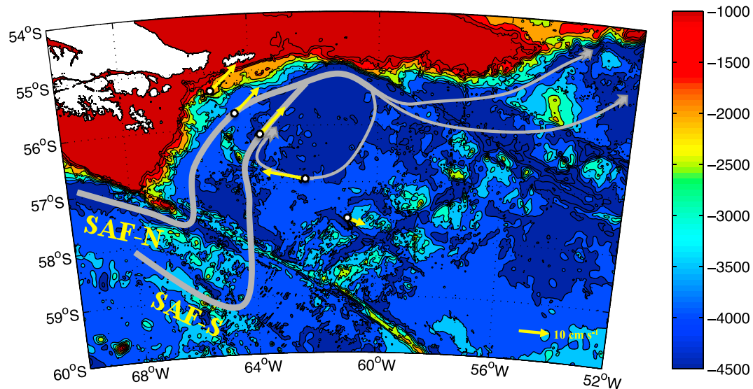
Figure 13. Schematics the permanent deep cyclonic circulation in the Yaghan Seafloor Depression. Velocities at mooring locations, indicated by yellow arrows, correspond to the mean values at the lower current meters. Velocity scale is indicated in the lower right corner. SAF-N: Subantarctic Front–Northern branch; SAF-S: Subantarctic Front–Southern branch.
