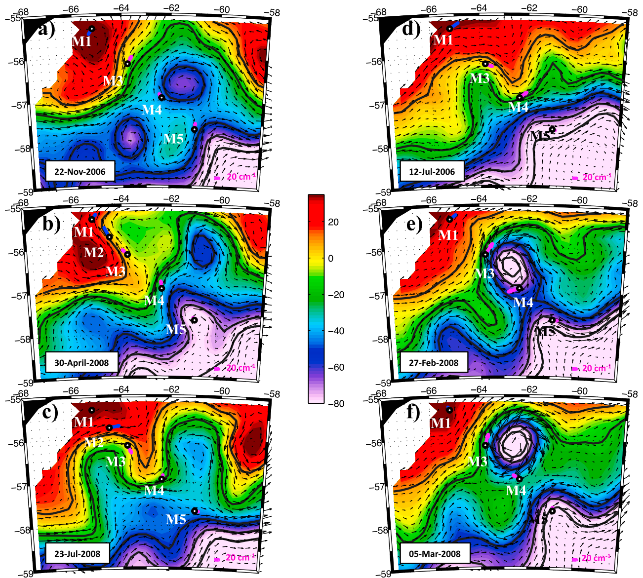
Figure 12. Maps of absolute dynamic topography of exceptional events studied in section 5.3 (in centimeters). The solid black lines are iso contours of absolute dynamic topography and correspond roughly to the mean positions of the frontal branches. For each mooring, the mean in situ velocity at 500 m depth is computed over 7 d centered on the date of each map and is shown by solid blue/rose arrows. Velocity scale is indicated in the lower right corner.
