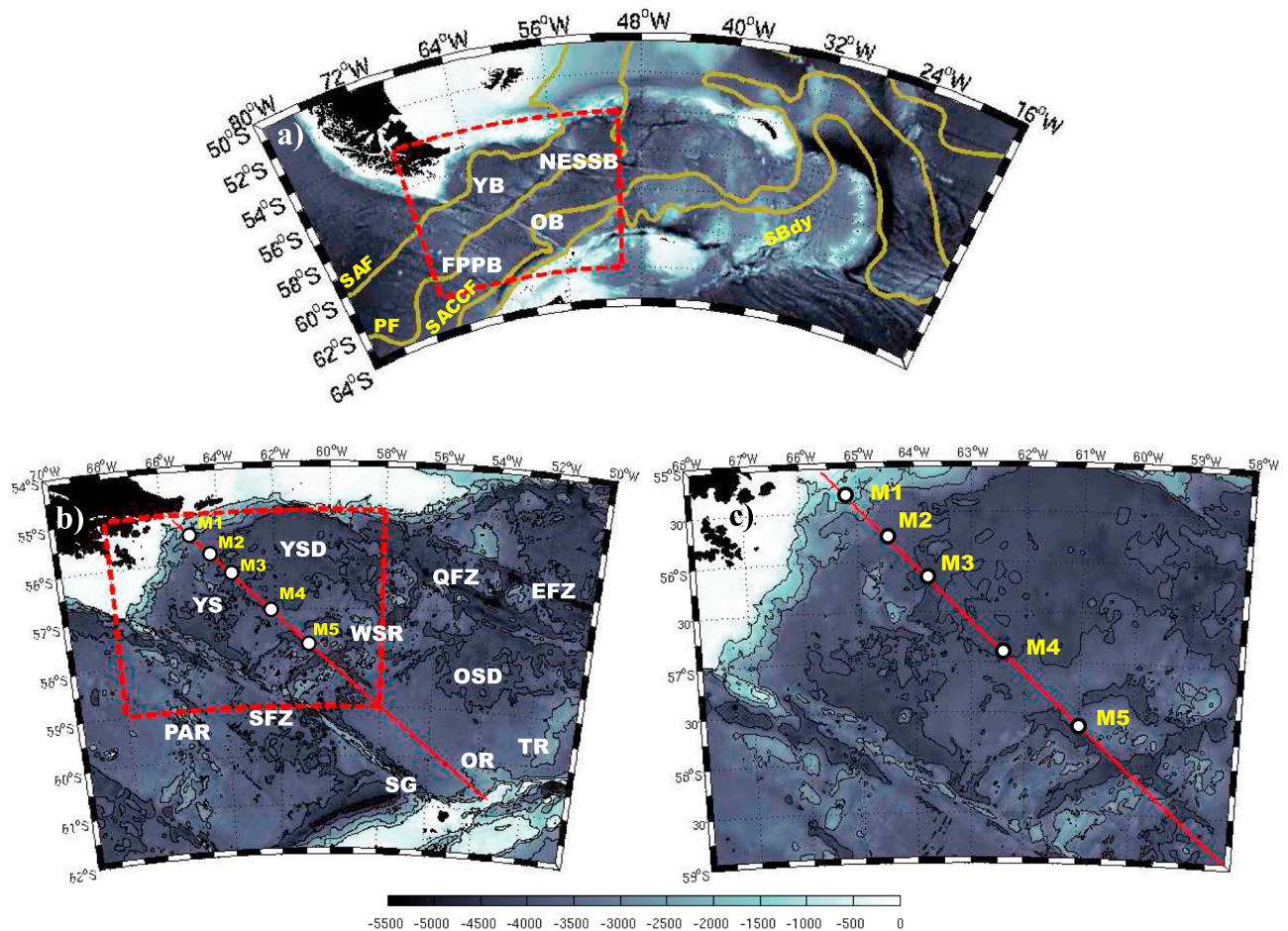
Figure 1. Bottom topography (in meters) and locations of the current meter moorings at Drake Passage. (a) Bottom topography of the Drake Passage with the main basins labeled: Yaghan Basin (YB), Ona Basin (OB), Former Phoenix Plate Basin (FPPB), and Northeast Scotia Sea Basin (NESSB). The yellow lines indicate the mean location of the major fronts, according to Orsi et al. [1995], from north to south: SAF, Subantarctic Front; PF, Polar Front; SACCf, South ACC Front; SBdy, southern boundary of the ACC. (b) White points indicate the locations of the moorings deployed along the Jason ground track 104 (red line) in the Yaghan Basin in January 2006. Major ridges or fracture zones are indicated: Shackleton Fracture zone (SFZ); Phoenix Antarctic Ridge (PAR); West Scotia Ridge (WSR); Ona Seafloor Depression (OSD); Ona Rise (OR) and Terror Rise (TR); Yaghan Seamounts (YS); Quest Fracture Zone (QFZ); Endurance Fracture Zone (EFZ); Yaghan Seafloor Depression (YSD); and the Shackleton Gap (SG). (c) Zoom on the mooring sites. Isobaths (1000, 2000, 3000, 4000 and 5000 m) are plotted.
