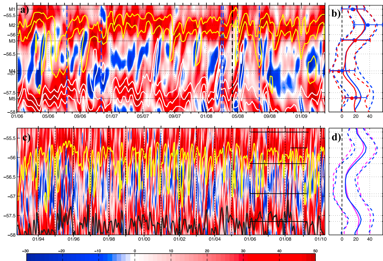
Figure 9. Time series of across-track velocities perpendicular to Jason track104 between 55.3°S and 58°S. (a) Time series of across-track surface geostrophic velocities derived from MADT between 18 January 2006 and 24 March 2009 and (c) for the period 1992–2011. Black horizontal lines indicate the mooring positions and their sampling duration. Vertical dashed blue and dashed black lines indicate the exceptional events studied in section 5.3. Color bar below indicates velocity in \text{cm s}^{-1} . In Figure 9a location of Subantarctic Front (SAF) branches are shown in yellow and location of Polar Front (PF) branches in white. In Figure 9c, for sake of clarity, only the locations of the southern branch of the SAF (yellow) and of the middle branch of the PF (black) are shown; they were calculated using a 28 d running mean of MADT. (b) Mean and standard deviation of the across-track component. Mean across-track velocity for MADT-based surface velocities over the period 2006–2009 is plotted in blue, and for the period 2008–2009 in red (solid: mean; dashed: mean plus or minus the standard deviation). The mean and standard deviation of the across-track velocity from in situ data for the periods 2006–2009 and 2008–2009 are plotted in blue and red dots, respectively. (d) Mean across-track MADT-based velocity for the period 1992–2011 is plotted in cyan, and the mean across-track velocity for the period 2006–2009 in blue (solid: mean; dashed: mean plus or minus the standard deviation).
