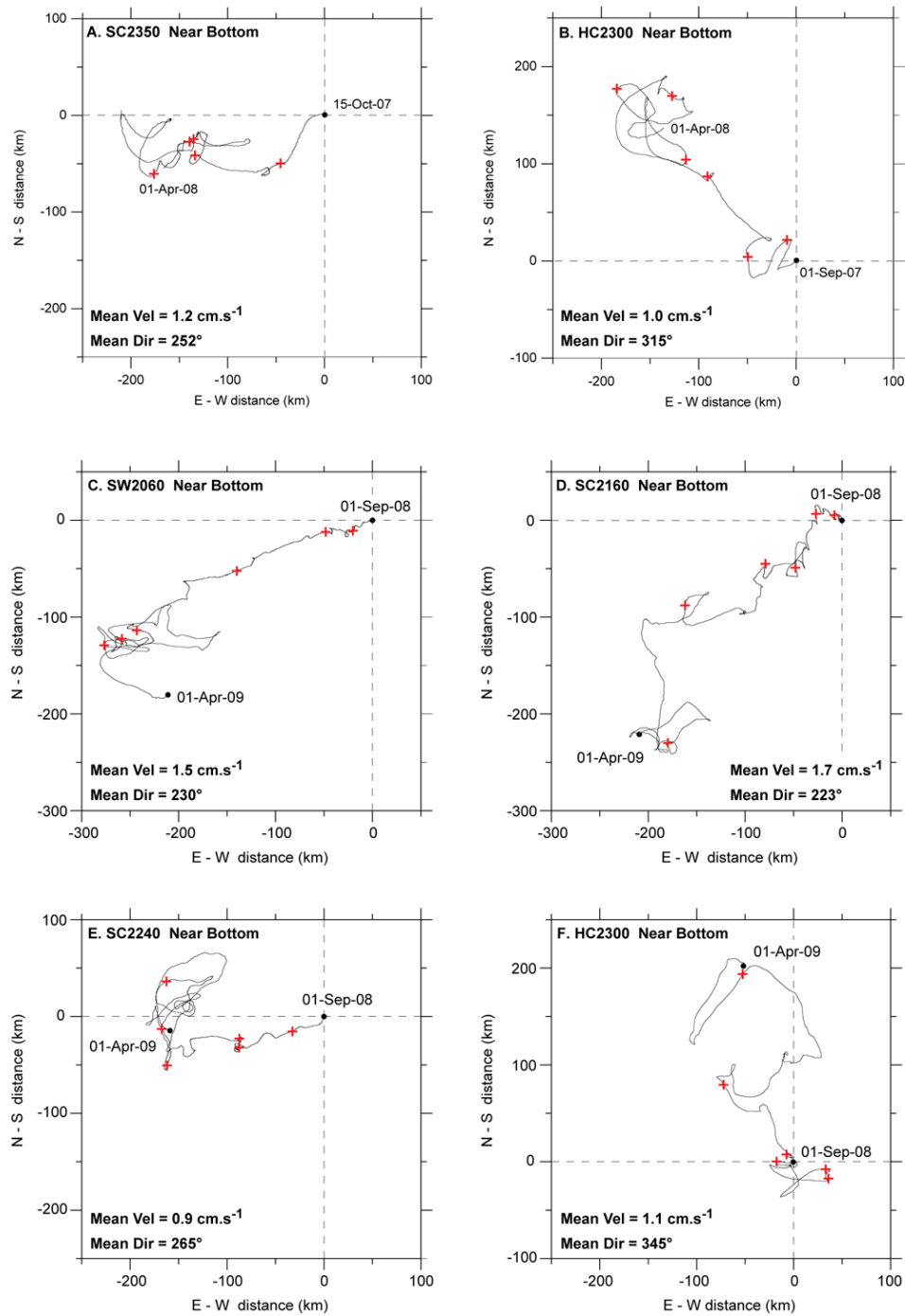
Fig. 7. Progressive vector diagrams of the near-bottom currents from September 2007 to April 2008 at SC2350 (A) and HC2300 (B), and from September 2008 to April 2009 at SW2060 (C), SC2160 (D), SC2240 (E), and HC2300 (F). Mean velocity and direction of the currents for the selected periods are indicated. Crosses represent time periods of one month.
