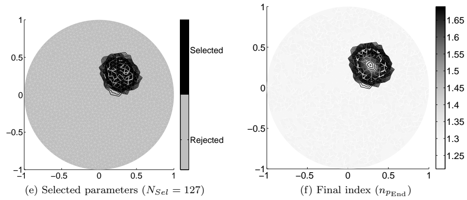
Figure 5: Selective reconstruction with 30 \times 30 data and \varepsilon = 2\% noise
