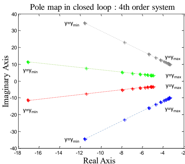
Figure 6: Pole evolution in closed loop for the 4 th order model at different equilibrium position
