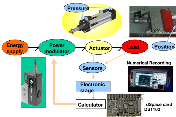
Figure 1: Experimental rig
