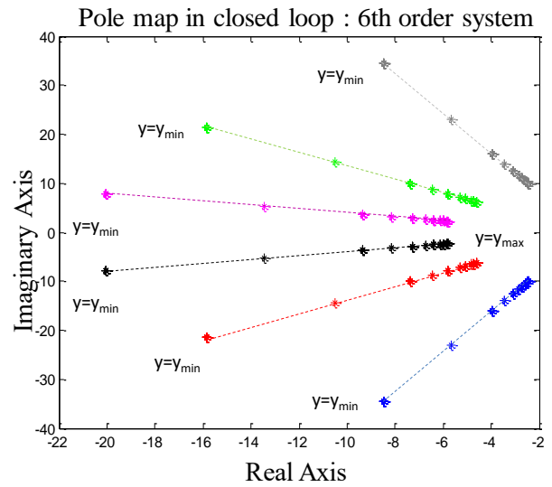
Figure 7: Pole evolution in closed loop for the 6 th order model at different equilibrium position
