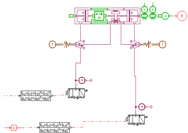
Figure 8: AMESim model
