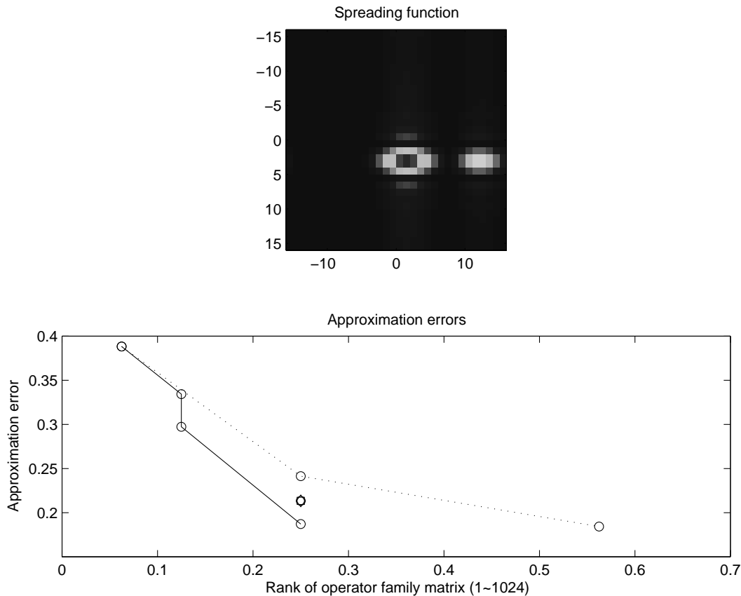
FIGURE 2. Approximation by Multiple Gabor Multipliers
