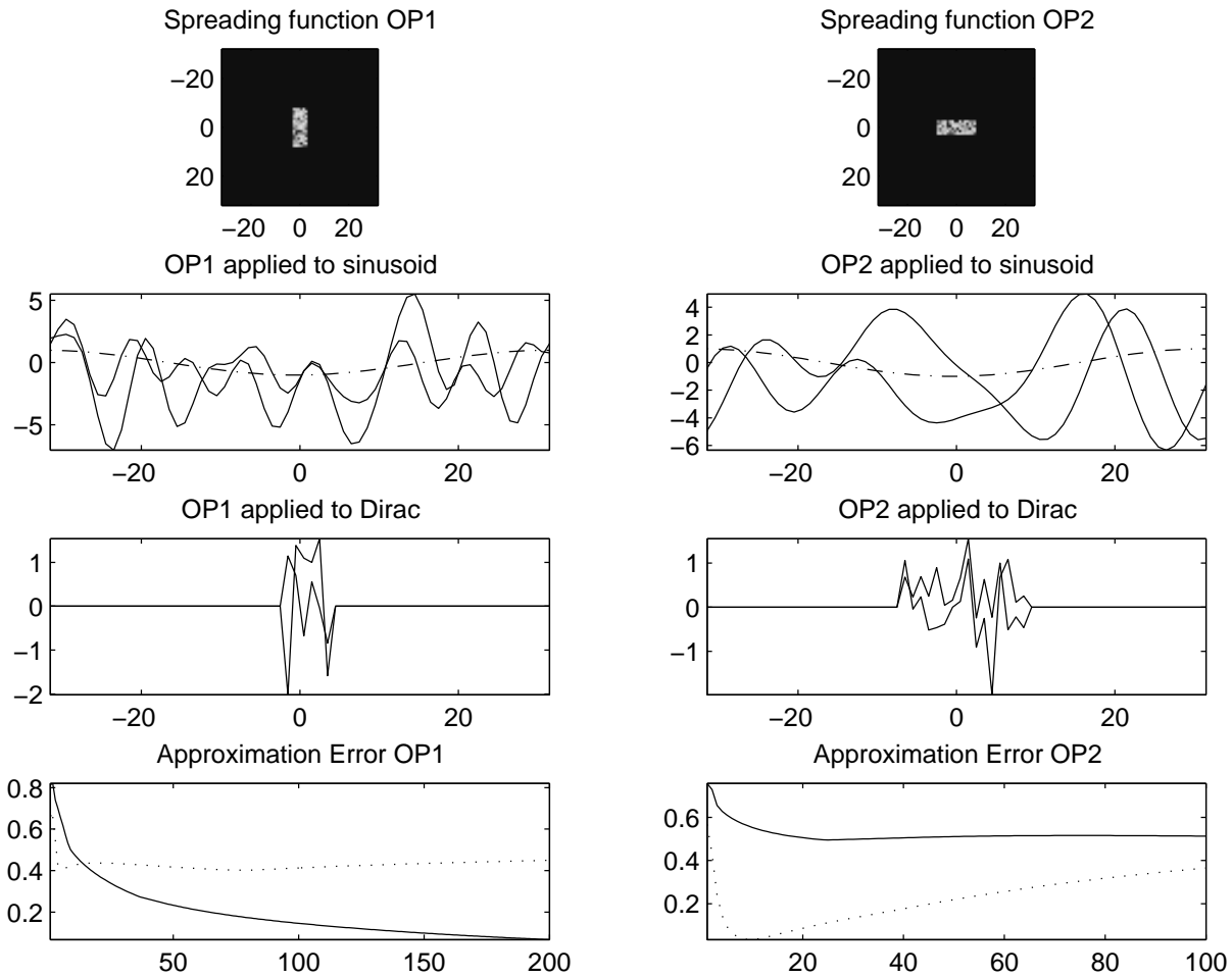
FIGURE 1. Approximation by Gabor Multipliers with parameters b_1, \nu_1 (solid) and b_2, \nu_2 (dashed)
