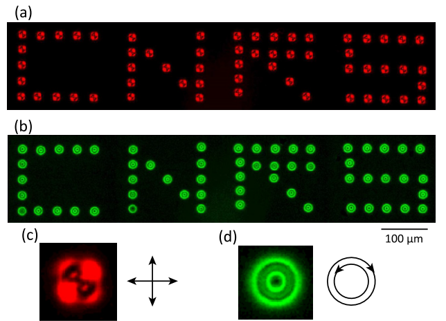
Figure 5. Demonstration of on-demand direct laser writing of arbitrary arrays of optical vortices. The four-letter acronym CNRS is observed between crossed linear polarizers at 633 nm wavelength (a) and between crossed circular polarizers at 532 nm wavelength (b). The enlargement of an individual pixel of each type is shown in panels (c) and (d), respectively, where arrows refer to the orientation of the polarizers.
