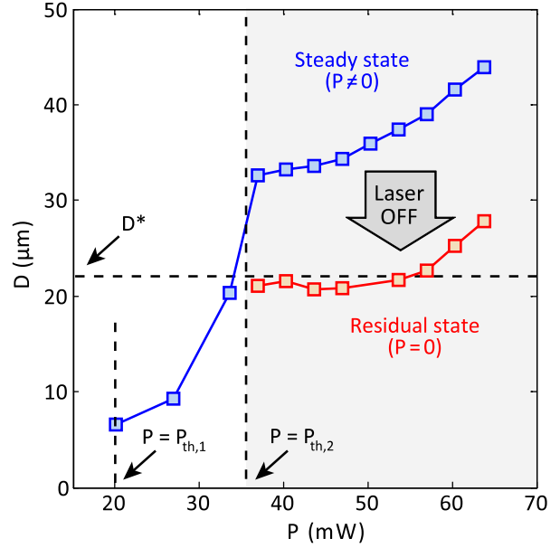
Figure 2. Diameter D of the light-induced reoriented director field versus the incident total power P . Above the threshold power P = P_{\text{th},2} , the top markers refer to the steady state under illumination whereas the bottom ones correspond to the residual state after the writing beam is turned off.
