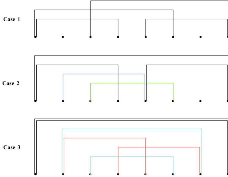
FIG. 1. Representation of the “extremal” situations in each case, that is, the \mathcal{B}_k ( k \in \{0, \dots, 4\} ). Each line connects the extremities of a block in \mathcal{B}_k . In case 2 (resp., case 3), the black lines are the ones common to \mathcal{B}_1 and \mathcal{B}_2 (resp., \mathcal{B}_3 and \mathcal{B}_3 ).
