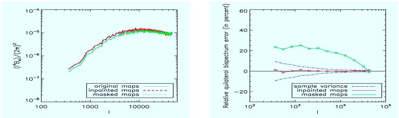
Figure 17. Bispectrum recovery for the Subaru mask.
