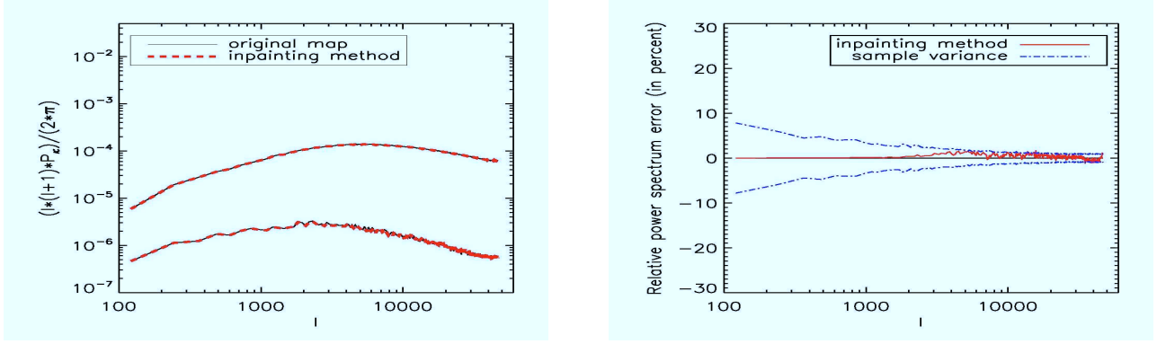
Figure 12. Power spectrum recovery from shear maps for CFHTLS mask: left, the two upper curves (almost superposed) correspond to the mean power spectrum computed from i) the complete simulated weak lensing mass maps (black - continuous line) and ii) the inpainted reconstructed maps from masked shear maps (red - dashed line), and the two lower curves are the empirical standard deviation for the complete maps (black - continuous line) and the inpainted reconstructed maps from masked shear maps (red - dashed line). Right, relative power spectrum error, i.e. the normalized difference between two upper curves of the left panel. The blue - dashed line represents the empirical standard deviation (cosmic variance) estimated from the complete mass maps.
