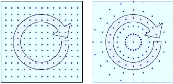
Figure 4. Calculation of the mean power per frequency using a regular grid (left) and using a polar grid (right)
