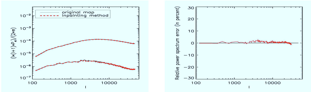
Figure 9. Power spectrum recovery from convergence maps for CFHTLS mask: left, the two upper curves (almost superposed) correspond to the mean power spectrum computed from i) the complete simulated weak lensing mass maps (black - continuous line) and ii) the inpainted masked maps (red - dashed line), and the two lower curves are the empirical standard deviation for the complete maps (black - continuous line) and the inpainted masked maps (red - dashed line). Right, relative power spectrum error, i.e. the normalized difference between two upper curves of the left panel.
