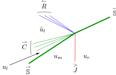
Figure 4: A 3-compression wave acting as a cancellation wave
