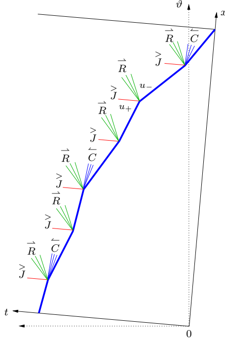
Figure 11: Beginning of Part 2
