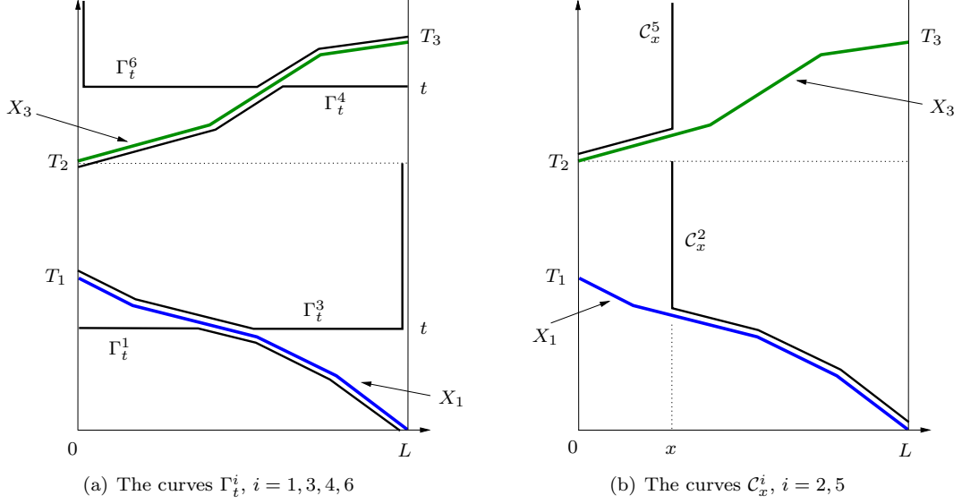
Figure 14: Curves for the BV estimate in the Lagrangian case
