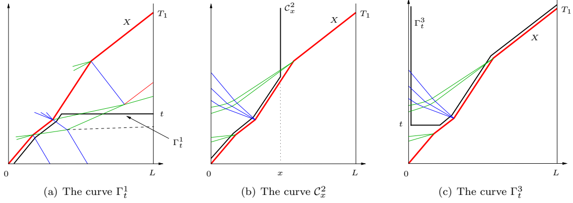
Figure 13: Curves for the BV estimate
