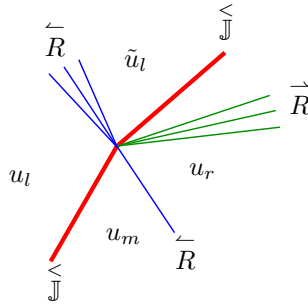
Figure 7: A 1-rarefaction crossing the 2-strong discontinuity
