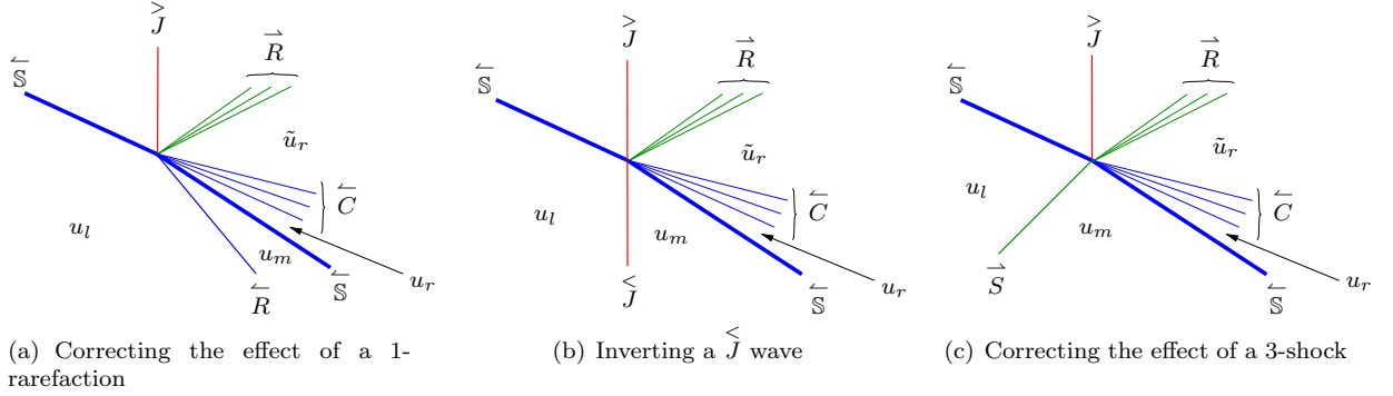
Figure 3: Compression waves acting as correction waves
