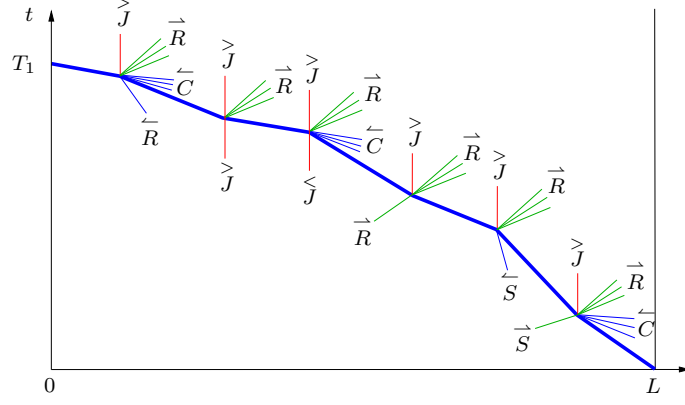
Figure 10: End of Part 1
