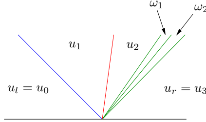
Figure 5: The accurate Riemann solver
