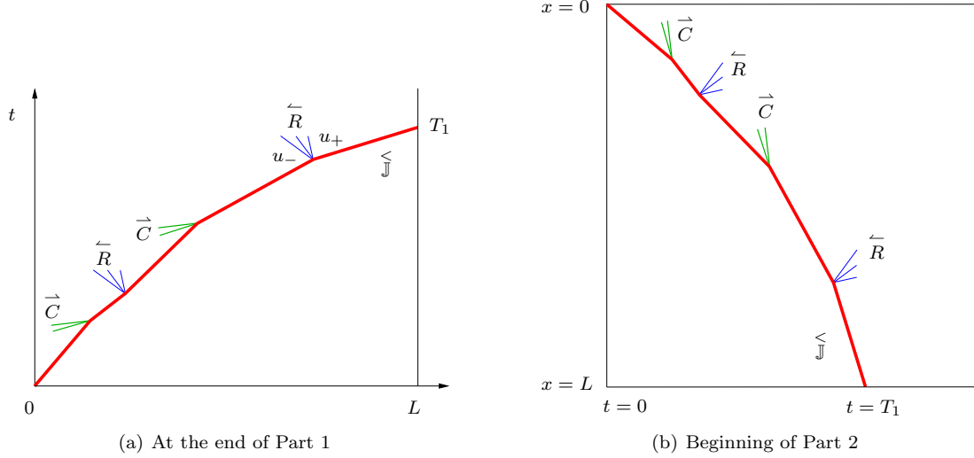
Figure 8: Junction of the two parts of the construction
