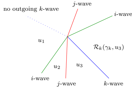
Figure 1: A cancellation k -wave
