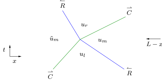
Figure 9: Simplified solver for side interactions
