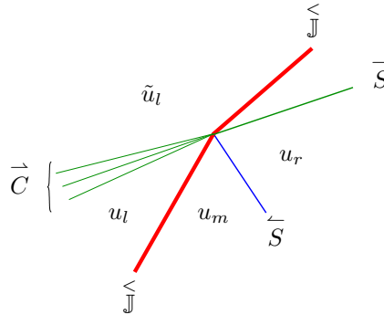
Figure 2: A 3-compression wave acting as a cancellation wave
