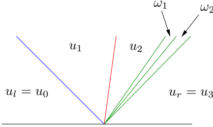
Figure 5: The accurate Riemann solver
