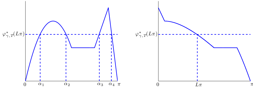
Figure 1: \Omega = (0, \pi) ; Graph of a function \varphi_{\gamma,T} (left) and graph of its decreasing rearrangement \varphi_{\gamma,T}^* (right). With the notations of the figure, \omega^* = (\alpha_1, \alpha_2) \cup (\alpha_3, \alpha_4) .
