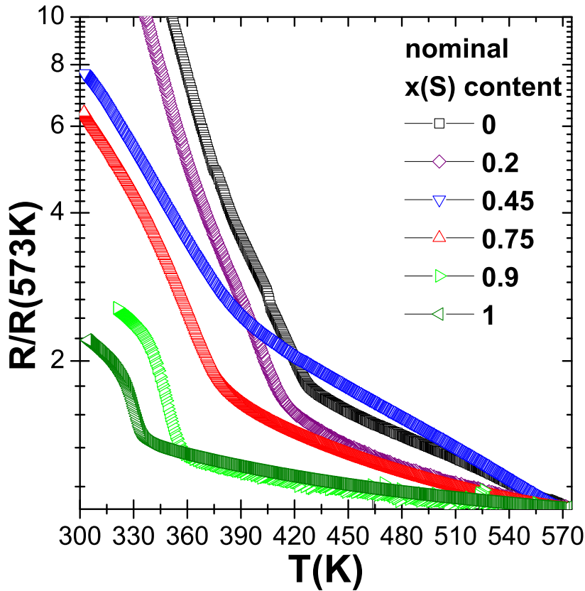
Figure 10. High temperature dependence of the electrical resistance of several Tl_{0.8}Fe_{1.5}(Se_{1-x}S_x)_2 samples with 0 \leq x \leq 1 . Nominal sulfur x(S) content is indicated. The anomaly related to the long range AFM structure in the ordered iron vacancies \sqrt{5} a \times \sqrt{5} a \times c network at T_N is clearly shown and decreases with x(S) .
