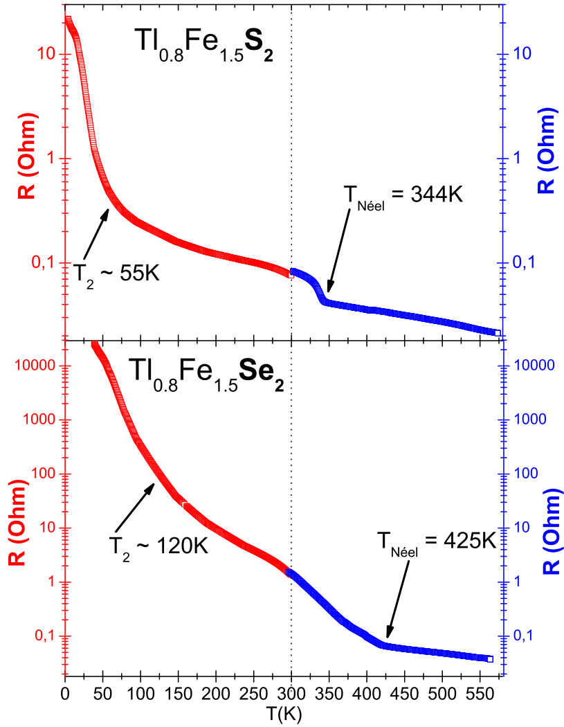
Figure 9. Low and high temperature dependence of the electrical resistance of typical x=0 and x=1.0 samples of the Tl_{0.8}Fe_{1.5}(Se_{1-x}S_x)_2 series emphasizing the signature of the long range AFM structure in the ordered iron vacancies \sqrt{5} a \times \sqrt{5} a \times c supercell at T_N .
