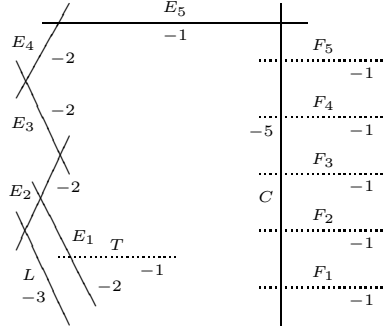
FIGURE 2.1. The total transform of \mu_*(C) \cup T \subset \mathbb{P}^2 in the minimal resolution \tau : \hat{V} \rightarrow V of \bar{q} . The plain curves correspond to the irreducible components of \tau^{-1}(D) and the exceptional divisors E_i of \tau are numbered according to the order they are extracted.
