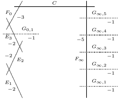
FIGURE 2.2. The total transform of F_0 \cup C \cup F_\infty \subset \mathbb{F}_n in X . The plain curves correspond to irreducible components of the boundary divisor B .
