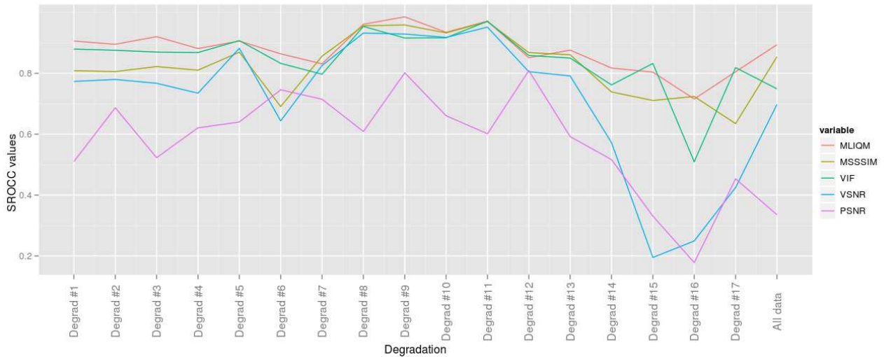
Figure 4. Obtained Spearman rank order correlation coefficient (SROCC) between the predicted DMOS values and the subjective DMOS scores considering TID2008 database as test set. The type of degradations are described in table 1.
