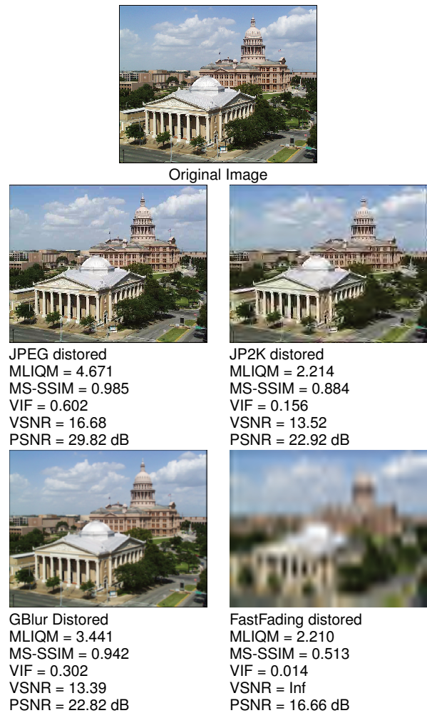
Figure 3. Example of results obtained computing the trial FR-IQA algorithms on an original image ( churchandcapitol extracted from LIVE and its degraded versions by applying JPEG (0.83865 bpp), JPEG2000 (0.194 bpp), Gaussian Blur ( \sigma = 1.565074 ) and a fast fading process (receiver SNR=18.9).
