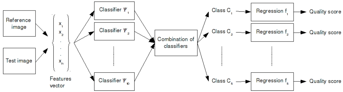
Figure 1. General scheme of the proposed method to obtain the final quality score of a test image.
