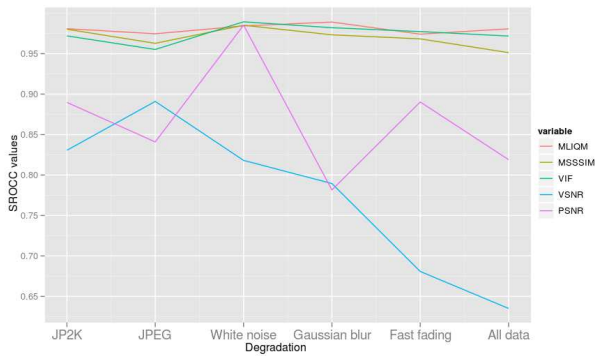
Figure 2. Obtained correlation coefficients between the predicted DMOS values and the subjective DMOS scores considering LIVE database test set.
