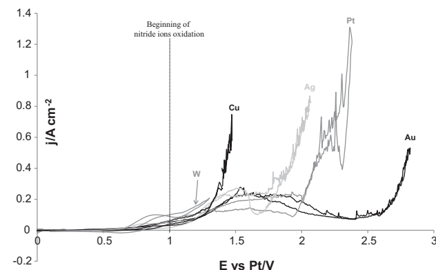
Fig. 3. Comparison of cyclic voltammograms in \text{LiF-CaF}_2\text{-Li}_3\text{N} ( 0.105 \text{ mol kg}^{-1} ) on several electrode materials at 1113 K and 100 \text{ mV s}^{-1} . Aux el: vitreous carbon, Ref el: Pt.
