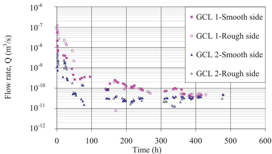
Figure .5 Comparisons between interface transmissivity results of the two faces of the bituminous GM
