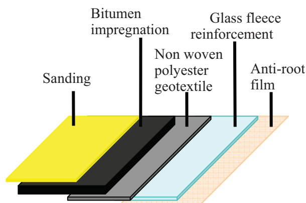
Figure 1. Typical cross-section of a BGM (adapted from Breul et al. 2008)
