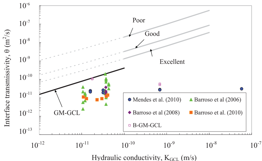
Figure 6. Synthesis of transmissivity data obtained in the literature for GCLs in contact with GMs and for B-GM in contact with GCLs obtained in this study
